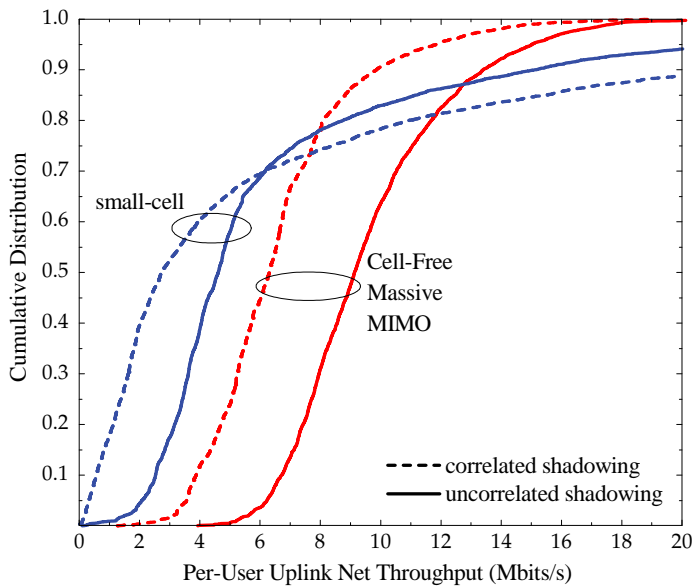
Fig. 4. The same as Figure 3 but for the uplink, and \tau^{\text{cf}} = \tau_{\text{u}}^{\text{sc}} = 20 .
