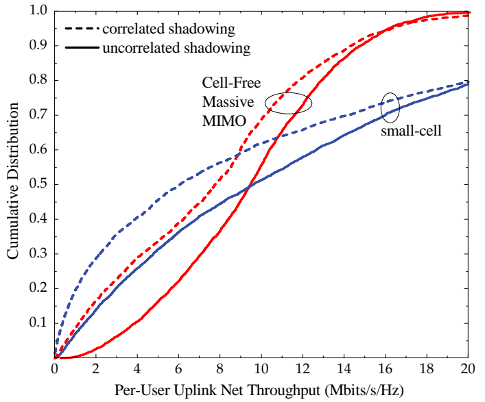
Fig. 6. The same as Figure 5 but for the uplink, and \tau^{\text{cf}} = \tau_{\text{u}}^{\text{sc}} = 20 .
