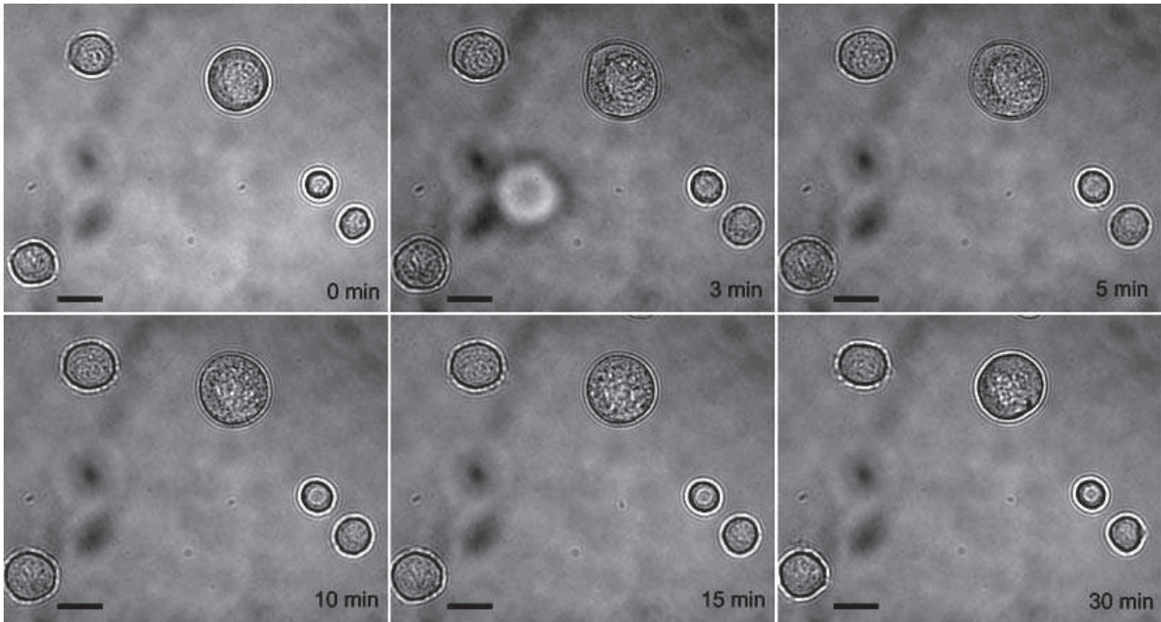
Figure 1. Swelling and regulatory volume decrease of B16-F1 cells in 100 mOsm buffer containing sucrose as the major osmolyte. The images show the same cells before (0 min) and during the hypotonic treatment at the indicated time intervals. After the rapid change of isotonic to hypotonic buffer at zero time, the cells swelled within 5 min and then shrank gradually within the observed time (5-30 min). Scale bar corresponds to 30 \mu\text{m} .
