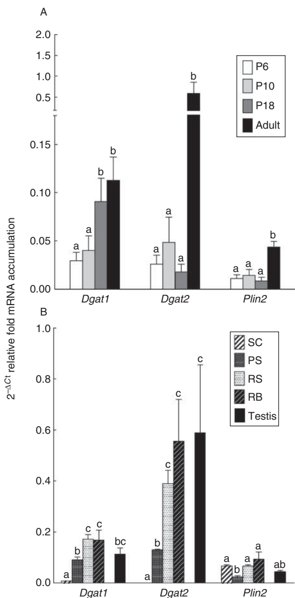
Figure 4 RT-qPCR analyses of Dgat1 , Dgat2 , and Plin2 transcripts during postnatal development in the mouse testis (A) and in cells from the seminiferous epithelium of adult mice (B). Data were normalized to Ppia and H2afz as internal reference using the 2^{-\Delta C_t} method. Values with different letters are significantly different ( P < 0.05 ). Statistical significance between different expression rates of all genes studied in a particular postnatal day or cell type is shown in Supplementary Table 1. SC, Sertoli cells.
