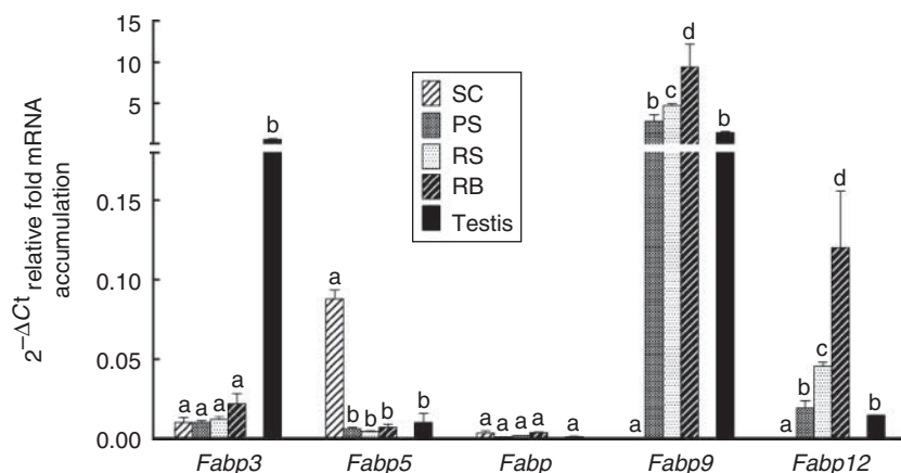
Figure 2 RT-qPCR analyses of Fabp3 , Fabp5 , Fabp7 , Fabp9 , and Fabp12 transcripts in different cell types purified from mouse seminiferous tubules. Data were normalized to Ppia and H2afz as internal reference using the 2^{-\Delta\Delta C_t} method. Values with different letters (a, b, c and d) are significantly different ( P < 0.05 ). Statistical significance between different expression rates of all genes studied in a particular cell type is shown as Supplementary Table 1 . SC, Sertoli cells.
