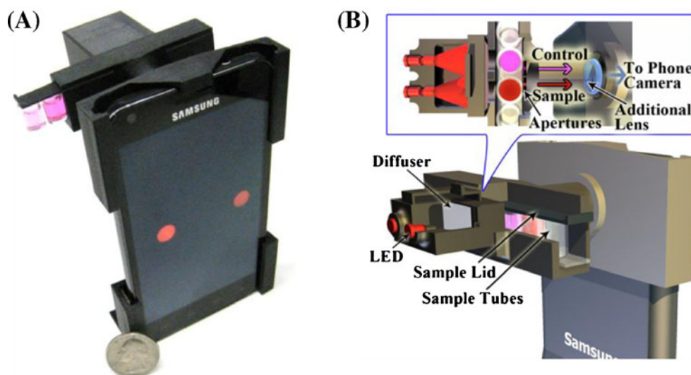
Fig. 1 a Cellphone-based digital reader for colorimetric assays on iTube platform [5]. The opto-mechanical attachment (~22 × 67 × 75 mm) that is installed at the back of the cellphone. b Schematics of the iTube platform. The iTube hardware attachment uses two interchangeable LEDs to illuminate the test and control tubes. Two diffusers are also inserted between the LEDs and the tubes to uniformly illuminate each tube. The transmitted
