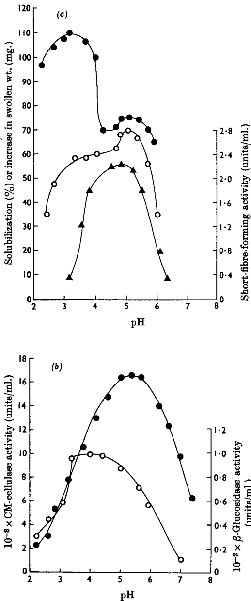
Fig. 4. Effect of pH on enzymic activity towards cotton, CM-cellulose and o -nitrophenyl \beta -D-glucoside. Activity towards cotton, shown in (a), was measured as S-factor (●), solubilization (▲) and short-fibre formation (○). Assays were carried out in 0.2M-acetate buffer (HCl-acetic acid for pH values 2.2–3.2 and acetic acid-NaOH for the remainder). Measurements of CM-cellulase (●) and \beta -glucosidase (○) activities, shown in (b), were carried out in phosphate-citrate buffer (0.1M-citric acid-0.2M- \text{Na}_2\text{HPO}_4 ). CM-cellulase and \beta -glucosidase showed the same pH optima when assayed in 0.2M-acetate buffer (acetic acid-NaOH).
