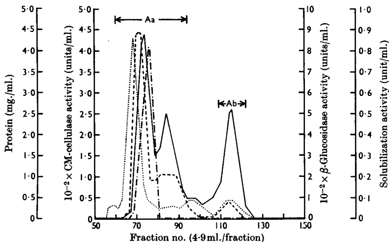
Fig. 5. Separation of a sample (5 ml.) of the concentrated culture filtrate [20–80% saturated (\text{NH}_4)_2\text{SO}_4 fraction redissolved to give a 50-fold concentration] on a column (100 cm. \times 3 cm.) of Sephadex G-75, the eluent being 0.1 M-acetate buffer (acetic acid–NaOH), pH 5.0. —, CM-cellulase; - - - - , \beta -glucosidase; ..... , protein; - · - · - · , solubilization. Assays were done as stated in the text. In a similar fractionation, fractions 60–94 (designation portion Aa, in the text) were combined as well as fractions 109–122 (portion Ab), and assays for recovery of cellulase (solubilization) and S-factor activity were carried out on these portions. Results are shown in Table 1.
