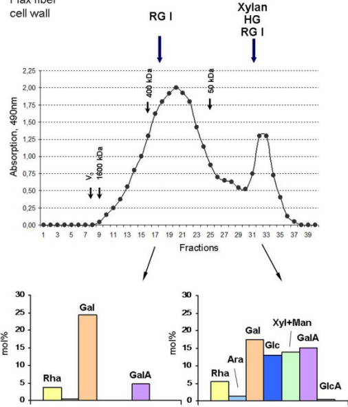
Figure 4. Elution profiles of polysaccharides strongly retained by cellulose microfibrils in the xylan and gelatinous cell walls and the relative monosaccharide content (mol%) of the main fractions of these polysaccharides.
