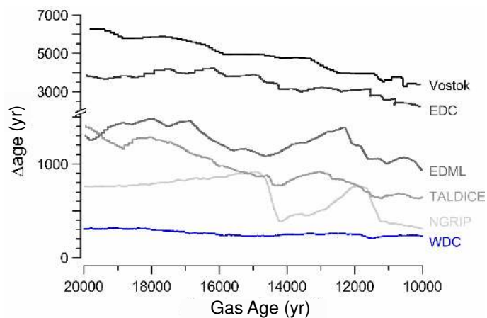
Extended Data Figure 4 | Calculated \Delta age offsets across the last deglacial termination for five ice cores from Antarctica and Greenland, compared with WDC. EDML, EPICA Dronning Maud Land; TALDICE, Talos Dome Ice; NGRIP, North Greenland Ice Project. Ice-core data from refs 58, 59.
