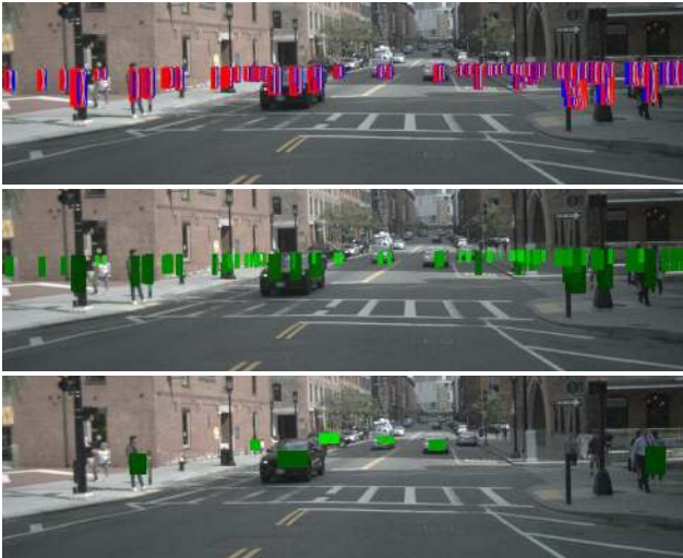
Figure 4. Expanding radar points to 3D pillars (top image). Directly mapping the pillars to the image and replacing with radar depth information results in poor association with objects’ center and many overlapping depth values (middle image). Frustum association accurately maps the radar detections to the center of objects and minimizes overlapping (bottom image). Radar detections are only associated to objects with a valid ground truth or detection box, and only if all or part of the radar detection pillar is inside the box. Frustum association also prevents associating radar detections caused by background objects such as buildings to foreground objects, as seen in the case of pedestrians on the right hand side of the image.
