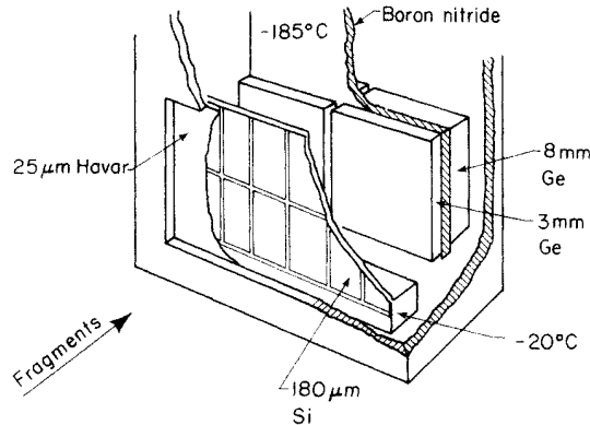
FIG. 3. Si-Ge telescope consisting of an array of 12 Si detectors, two thin Ge and two thick Ge detectors enclosed in a cryostat. The boron nitride had the shape of a window frame. The telescope had an active area of 20 \text{ cm}^2 .
