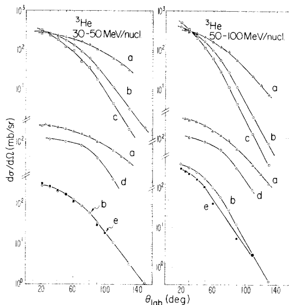
FIG. 14. Cross comparison of angular distributions of {}^3\text{He} fragments integrated for two velocity windows at different incident energies and for different projectiles and targets: (a)–(c) Ne on U at 2.1, 0.4, and 0.25 GeV/nucleon, respectively; (d) Ne on Al at 2.1 GeV/nucleon (raised by a factor of 10); and (e) {}^4\text{He} on U at 0.4 GeV/nucleon (raised by a factor of 10).
