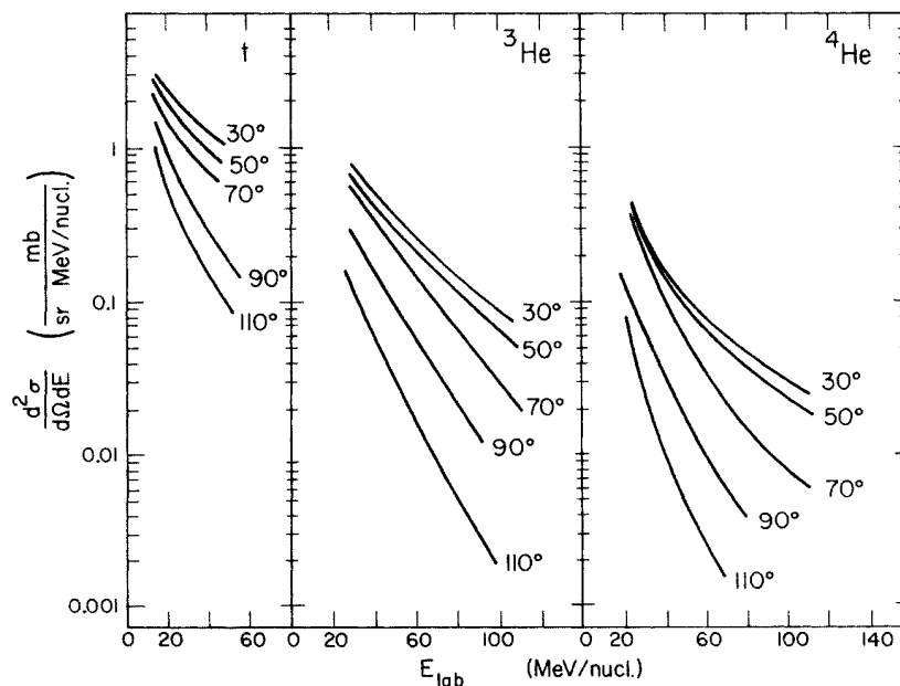
FIG. 11. Triton, {}^3\text{He} , and {}^4\text{He} double differential cross sections from the irradiation of aluminum with 2.1 GeV/nucleon {}^{20}\text{Ne} ions.
