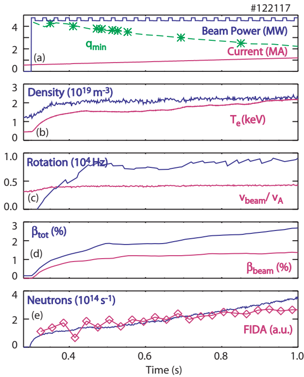
Figure 2. Time evolution of (a) neutral beam power, plasma current, and q_{\text{min}} inferred from the RSAE cascades, (b) line-average electron density \bar{n}_e and central electron temperature, (c) central toroidal rotation from charge-exchange recombination spectroscopy of carbon impurities and ratio of the speed of injected 81 keV deuterium ions to the Alfvén speed evaluated using the vacuum magnetic field (2.0 T) and \bar{n}_e , (d) central toroidal beta and central beam-ion beta from TRANSP assuming neoclassical fast-ion behaviour and (e) measured neutron rate and FIDA density at 1.94 m in the baseline discharge.
