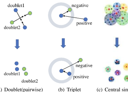
Figure 1. The intuition behind pairwise/triplet similarity based hashing methods and the proposed center similarity quantization. Pairwise and triplet learnings only consider a pair/triplet of data at once, while our central similarity encourages all similar data points to collapse to the corresponding hash centers (red stars).
