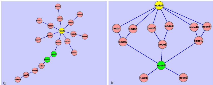
Fig. 2. a. The network shows the difference between eccentricity and closeness. The values of eccentricity are node0=0.14 , node8=0.2 , node15=0.2 . The closeness values are node0=0.021 , node8=0.017 , node15=0.014 . In this case node0 is closer than node8 and node15 to the most of nodes in the graph. Eccentricity value of node0 is smaller than value of node8 and node15 , but this is due only to few nodes. If they are proteins this probably mean that node0 is fundamental for the most of reaction in the network, and that node8 and node15 are important only in reactions between few proteins. b. The network shows the difference between centroid and closeness. Here node0 has highest centroid value (centroid=1, closeness=0,04) and node7 has highest closeness value (centroid=-1, closeness= 0,05).
