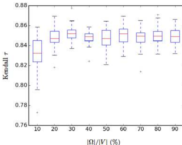
Figure 4: Correlation scores for expected versus realized centrality for SOC-betweenness centrality for the Minnesota state road network. Each boxplot represents 30 random choices of the set \Omega , with \kappa = 20
