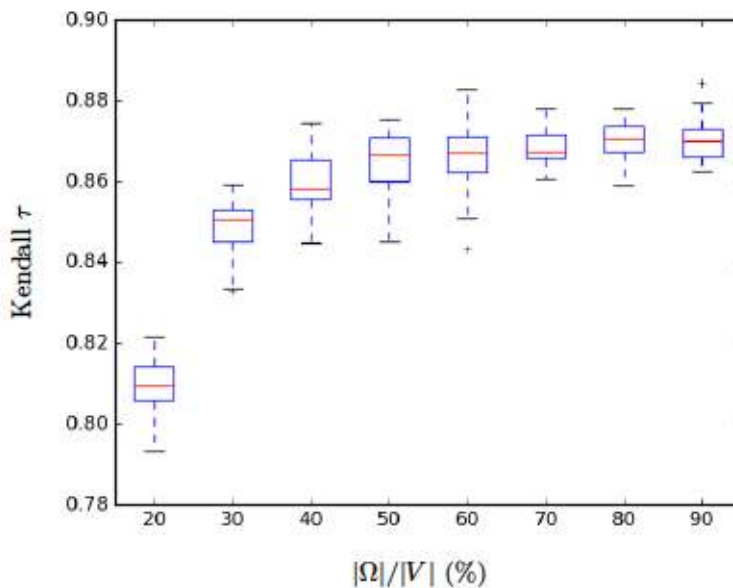
Figure 2: Correlation scores for expected versus realized centrality for SOC-betweenness centrality for the Gnutella network. Each boxplot represents 30 random choices of the set \Omega , with \kappa = 4
