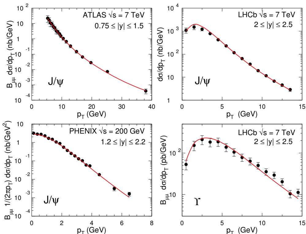
Figure 1. Comparison between heavy-quarkonium ( J/\psi , \Upsilon ) production data in p-p collisions and the parametrization (2.11) (solid red line). Data are taken from ATLAS [24], LHCb [25, 26], and PHENIX [27].
