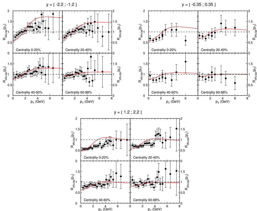
Figure 4. Same as figure 3 in the four centrality classes (from top left to bottom right in each panel) at backward, central and forward rapidities (upper left, upper right, bottom).
