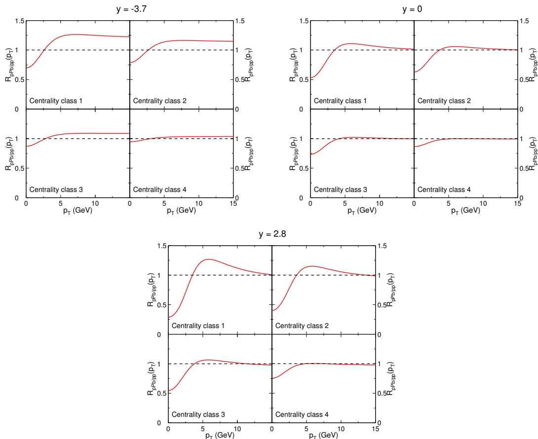
Figure 6. Same as figure 5 in the four centrality classes (from top left to bottom right in each panel) at backward, central and forward rapidities (upper left, upper right, bottom).
