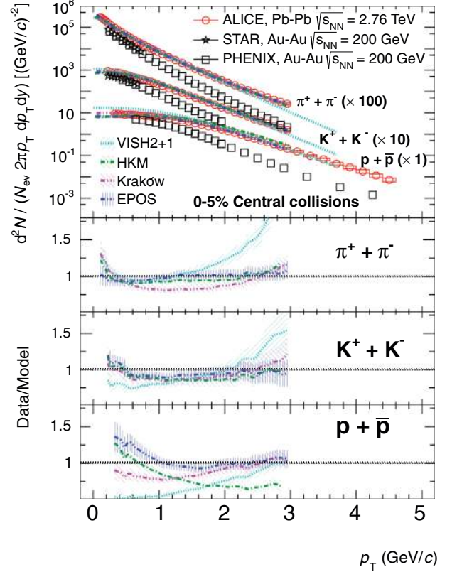
FIG. 13. (Color online) Spectra of particles for summed charge states in the centrality bin 0–5% compared to hydrodynamical models and results from RHIC at \sqrt{s_{NN}} = 200 GeV [42,45]. See text for details. Systematic uncertainties plotted (boxes); statistical uncertainties are smaller than the symbol size.
