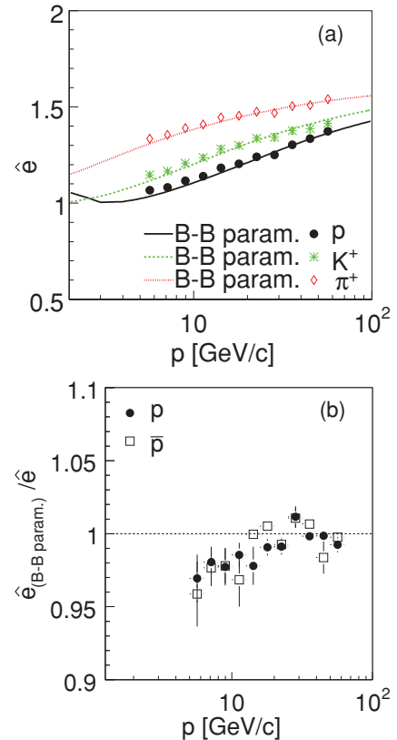
FIG. 1. (Color online) (a) The most probable specific energy loss \hat{e} for particle species \pi^+, K^+ , and p as a function of total momentum p . The points show results extracted from data, whereas the lines indicate the Bethe-Bloch parametrizations optimized for the NA49 measurement. (b) The ratios of the Bethe-Bloch parametrizations ( \hat{e}_{B-B\text{param.}} ) to \hat{e} from fits to the data are shown as a function of laboratory momentum.
