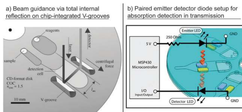
Fig. 9 Different setups for optical detection. (a) Enhancement of sensitivity by on-chip beam guidance using chip-integrated V-grooves. 149 (With kind permission from Springer Science and Business Media.) (b) Paired emitter detector diode (PEDD) setup as sensitive and cheap alternative to common LED–photodiode setups for absorption measurement in transmission. 117 (Reproduced with permission from The Royal Society of Chemistry.)
