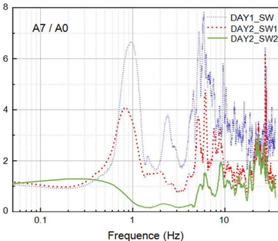
Fig. 2. Spectrum ratios of motions (A7 and A0)
