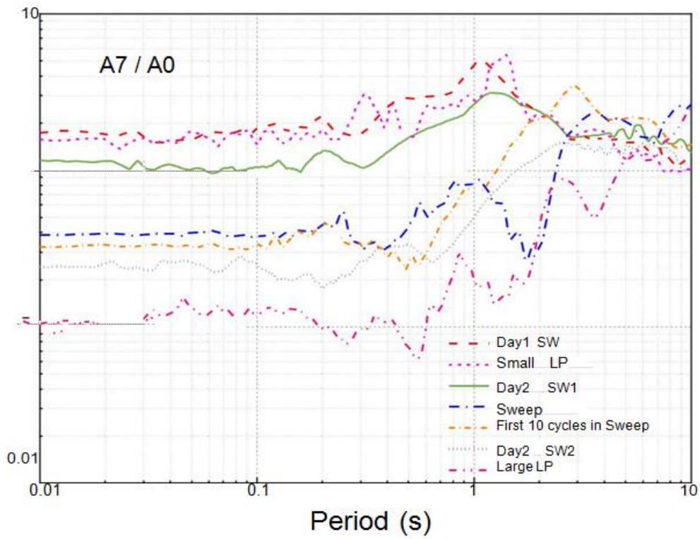
Fig. 4. Response spectrum ratio of accelerations during all shaking events
