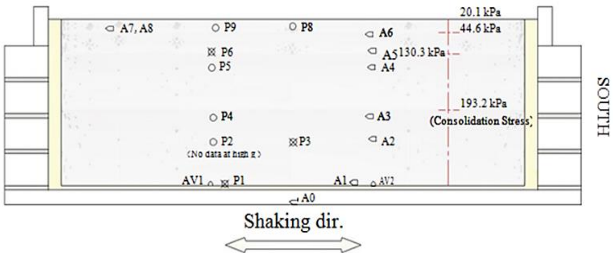
Fig. 1. Instrumental Arrangements in centrifuge model
