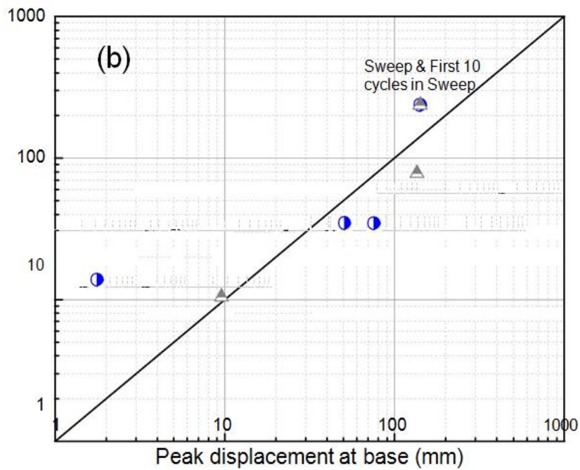
(b) Peak displacement
