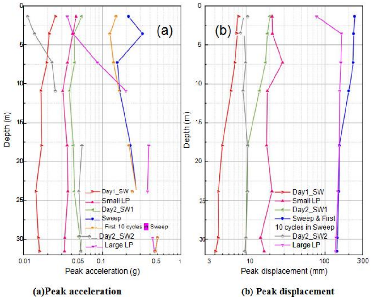
Fig. 5. Depth profiles of peak acceleration and peak displacement for all shaking events
