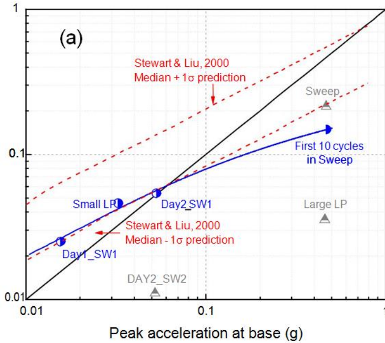
(a) Peak acceleration
