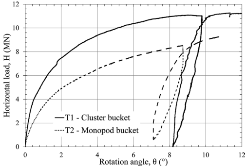
Figure 4. Load-displacement curves of cluster and monopod bucket foundations.
