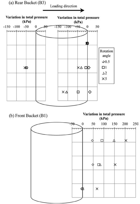
Figure 8. Distributions of total pressure deviations at rotation angles of 0.5^\circ , 1^\circ , 2^\circ , and 5^\circ .
