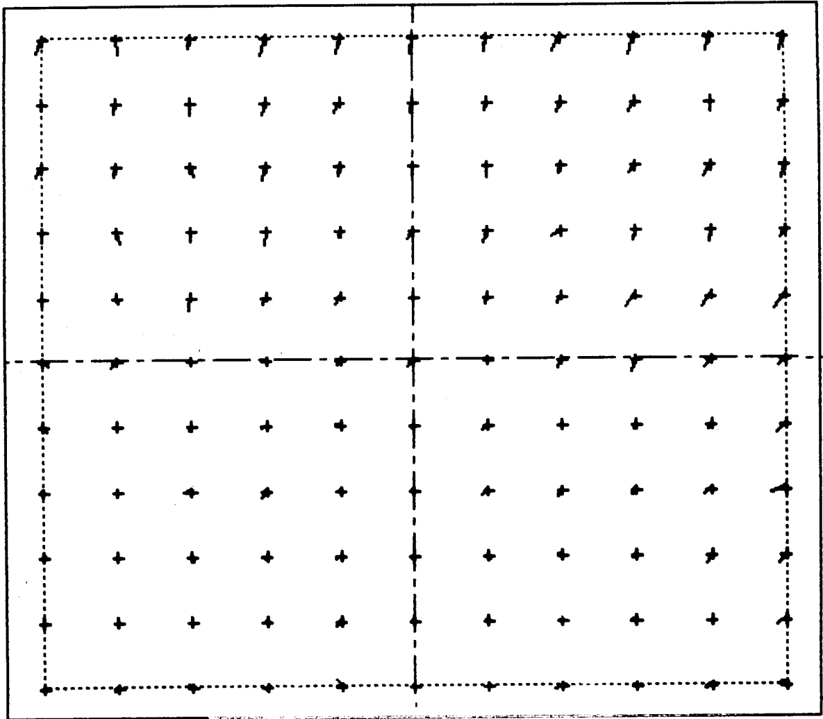
Fig. 45 Pixel Performance Map - Conical PSF and Good CCD
