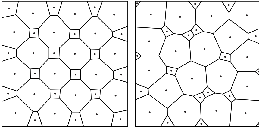
FIG. 2. CPDs of 36 points with density \rho = 1 . In the first example (left) the 18 small cells have weights w \approx -0.01389 , and the 18 large cells have weights w = 0 . In the second example (center) the 18 small cells have weights w \approx -0.01667 , and the 18 large cells have weights w = 0 . Both diagrams were obtained by applying a modified form of Lloyd's algorithm (in which the locations are updated to the centroids but the weights are fixed) to an initial checkerboard pattern in which the generators lie on a square lattice with an alternating pattern of weights. Both examples are fixed points of Algorithm 1 with an appropriately constructed f .
