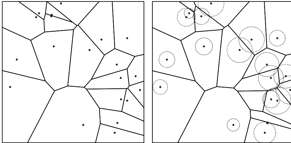
FIG. 1. A comparison of a standard Voronoi diagram (left) with a power diagram (right). The location of the generators in both cases is the same, but the power diagram carries additional structure via the weights associated with each generator. The size of the weights in the power diagram is indicated by the radii of the dashed circles. Notice that in the power diagram it is possible for the generator to lie outside the cell or for the cell associated with a generator to be empty (the Voronoi diagram has 20 cells, and the power diagram has 19 cells). The geometrical construction of the power diagram in terms of the generator locations and the circles is simple; for each point \mathbf{x} construct a tangent line from \mathbf{x} to the circles centered at \mathbf{x}_i with radii r_i ; the length of the tangent line is called the power of the point \mathbf{x} , and the point \mathbf{x} belongs to the power cell that has minimum power. The weights of the generators in this case are w_i = r_i^2 .
