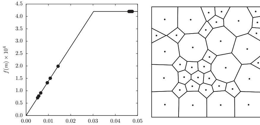
FIG. 3. The leftmost CPD in Figure 2 is a monotone CPD and is a critical point of the energy with appropriately constructed f . For this CPD, the construction of f following the proof of Proposition 2.11 gives the function f(m) shown here (left). As a test, our generalized Lloyd algorithm using this f was applied to a random initial configuration of 36 cells. The algorithm converged to the CPD with two different cell sizes shown above (right).
