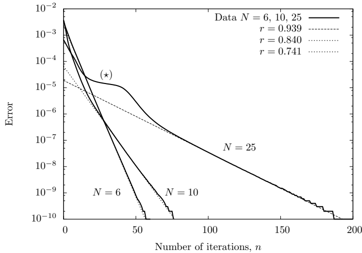
FIG. 6. Rate of convergence of the generalized Lloyd algorithm to critical points of the energy (4.1) with \lambda = 0.005 . The approximate deviation of the energy from its minimum against the number of iterations is plotted on semilog axes for three simulations, each using random initial conditions. The initial number of generators in the three cases was N = 6, 10, 25 , and there was no elimination of generators throughout the simulations. We see that the algorithm converges linearly with rate r . The rate was computed by fitting straight lines to the data.
