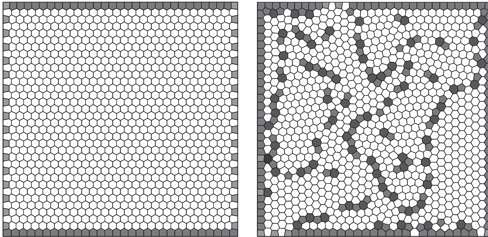
FIG. 5. Two local minimizers of the energy (4.1) for \lambda = 10^{-5} with N = 1037 in both cases. In the first case the cell generators were initially arranged in a triangular lattice; in the second case they were distributed randomly.
