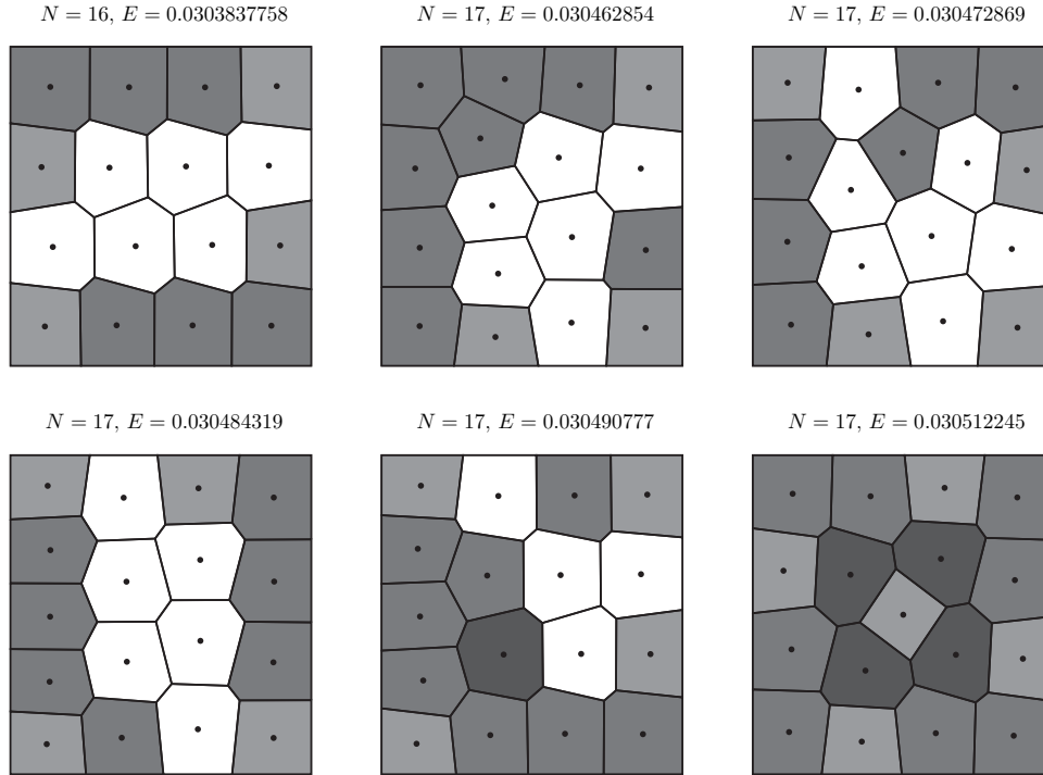
FIG. 4. Flatness of the energy landscape: Some local minimizers of the energy (4.1) for \lambda = 0.005 . The polygons are the power cells P_i , and the points are the generators \mathbf{x}_i . The weights w_i are not shown. The shading corresponds to the number of sides of the cells.
