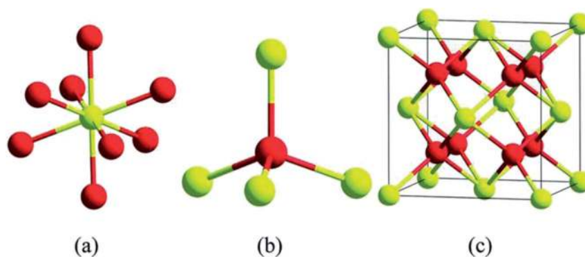
Fig. 2 Structurally analyzed ceria crystals \text{Ce}_4\text{O}_8 (unit cell); in (a) and (b) yellow color represents eight-folds of cerium atoms and red represents four-fold oxygen atoms in ceria crystal structure; (c) is the basic fcc fluorite lattice structure of \text{Ce}_4\text{O}_8 (reproduced from K. Reed et al. , Environ. Sci.: Nano , The Royal Society of Chemistry, 2014 (ref. 22)).
