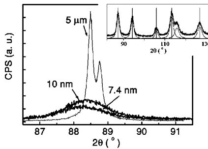
FIG. 4. X-ray spectra showing peak shift and peak broadening of 7.4 and 10 nm \text{CeO}_2 nanoparticles, compared with micron size particles ( \sim 5 micron). The small figure in the upper right-hand side corner shows the linewidth and lineshape fit of an x-ray diffraction pattern of 10 nm particles.
