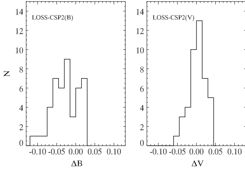
Figure 10. Histograms of the differences in the LOSS-CSP2 BV photometry for all the comparison stars in common between the two samples. The distributions are roughly symmetric in V but not in B .
