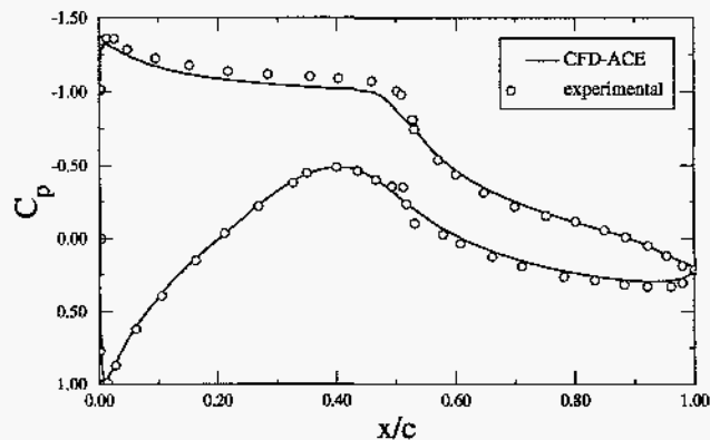
Figure 4. Pressure Distributions for \alpha = 5.13^\circ , Fully Turbulent Calculation
