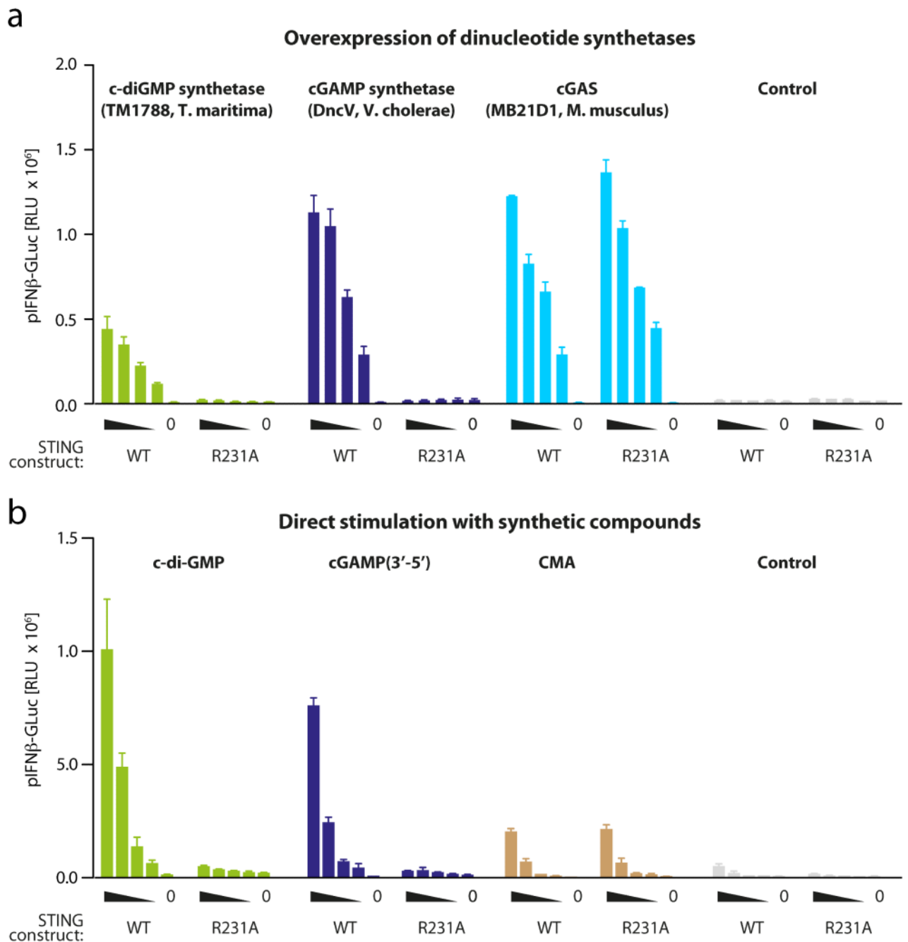
Figure 1. The R231A STING mutant uncouples cyclic di-GMP sensing from cGAS-induced activation
