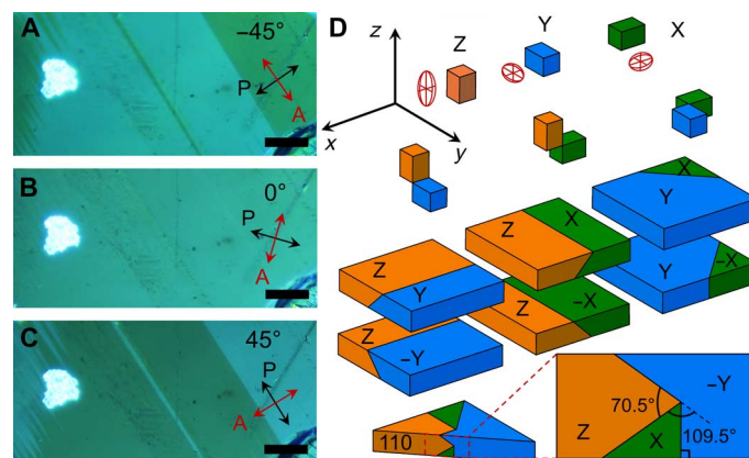
Fig. 1. Polarized light optical images and domain configurations in a MAPbI 3 single crystal (sample C). (A to C) Reflection-mode polarized optical micrographs (crossed Nicols) showing contrast reversal of domain groups as a function of sample rotation relative to the polarizer-analyzer (P-A) pair. At 0° relative angle, the domain groups are indistinguishable, and, at 45° and -45°, the domain contrast is maximum; that is, \theta_e = 90^\circ . The red and black arrows indicate the analyzer orientation and polarizer orientation, respectively. The light intensity of a bright dust particle is insensitive to the sample rotation. Scale bars, 5 \mu\text{m} . (D) Permissible domains of the MAPbI 3 tetragonal phase. At the cubic-to-tetragonal transition, the tetragonal unit cell can form with the c axis aligned along any of the three axes ( x , y , and z ) of the parental cubic phase, leading to three possible configurations ( X , Y , and Z ). To preserve crystal integrity, the a axes of different domains must coincide (32), leading to six possible domain orientations that are characterized by domain walls intersecting at 0°, 90°, or 45° in the principal planes of the parental phase and at \approx 70^\circ and \approx 110^\circ in the (110) plane.
