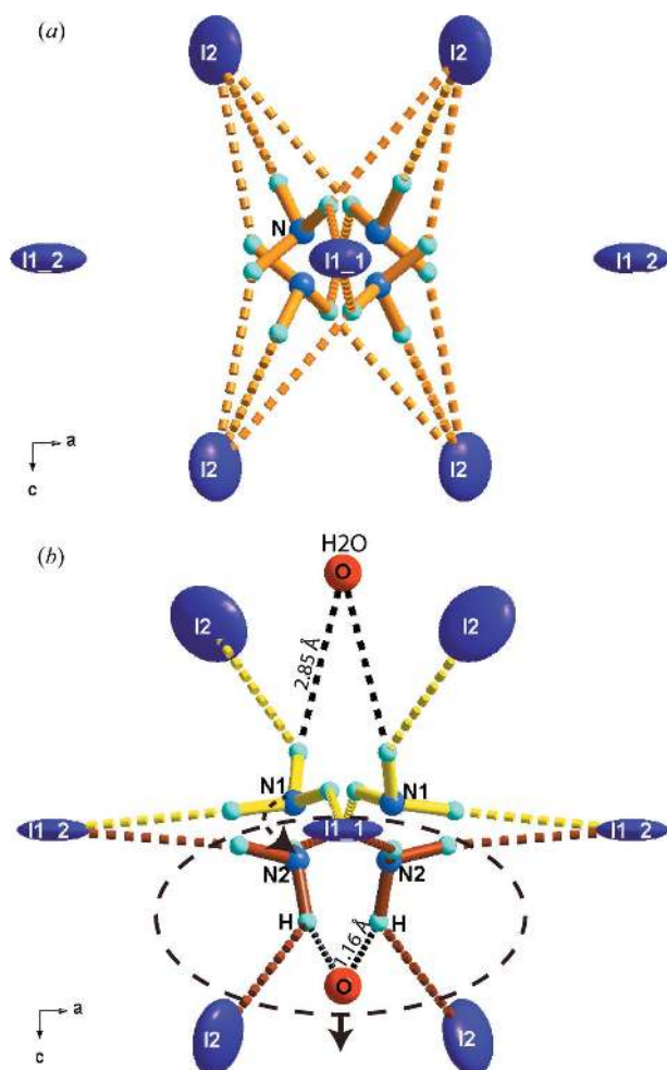
Figure 5 Comparison of the hydrogen bonds in (a) the pristine (I) and (b) the aged (II) crystals. The system of the N—H...I hydrogen bonds connecting the [CH 3 NH 3 ] + cation with the (Pb,I)-framework is shown. The four shown N atoms correspond to the four orientations of the cation. Three corresponding H atoms are shown for each N position. In (I) (a), all 12 hydrogen bonds (orange lines) are statistically present with a probability of 25% for each one. In (II) (b), six bonds (brown lines) corresponding to cation 2 (N2) are present with 29.5% probability and six bonds (yellow lines) corresponding to cation 1 (N1) are present with 16.5% probability for each. The O—H interactions (black dotted lines) are present with a probability of 8.8%. The probabilities of the bonds are defined by the probability of the cation orientations and the O occupancy. The dashed black contour indicates the most probable part of the structure, which leads to its decomposition. The dashed black arrow between N1 and N2 indicates the compensation of the leaving part.
