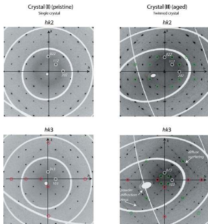
Figure 1 hk2 and hk3 reciprocal space sections of the pristine and aged crystals. Red circles surround some of the h03 and 0k3 reflections violating the condition h, k, l = 2n for 0kl and h0l reflections. These reflections are incompatible with the alternating c and b glide planes in the tetragonal space groups I4/mcm of both the pristine and aged crystals. Green circles surround some reflections violating the condition h + k + l = 2n . These reflections are incompatible with the I centring of the unit cell in the aged crystal. Diffuse scattering lines and powder diffraction rings are well visible in the aged crystal images.
