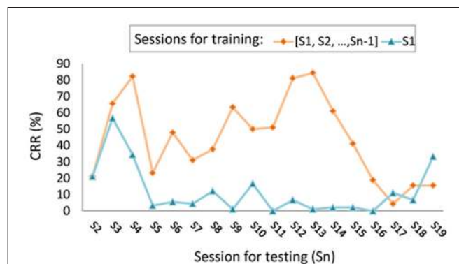
FIGURE 2 | Longitudinal variations in correct recognition rate (CRR) using two-stage person identification system with/without incremental learning, depicted by orange diamonds and blue triangles, respectively (figure depicted according to the results of self-paced finger movement experiment presented in our previous work, Cheng, 2013).
