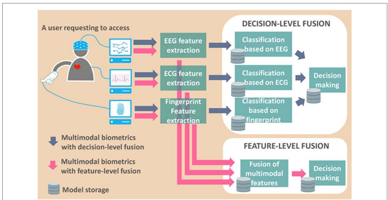
FIGURE 4 | Diagram of data processing flow in multimodal biometric system (enrollment procedure not shown).
