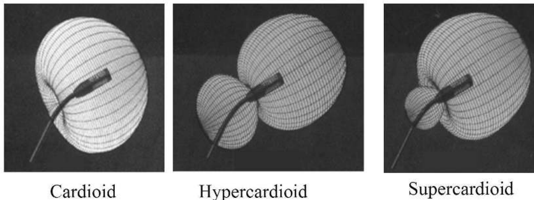
Figure 1. (A) The relationship between the ratio of the internal and external delays and the polar patterns. (Reprinted with permission from Powers and Hamacher, Hear J , 55[10], 2002). (B) The directional sensitivity patterns of directional microphones exhibiting cardioid, hypercardioid, and supercardioid patterns. A commercial stand directional microphone is placed at the center of the directional sensitivity pattern.
