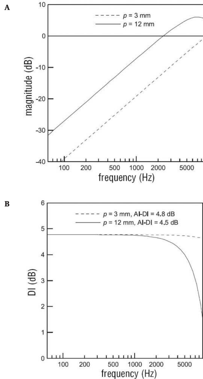
Figure 2. (A) The relationship between the port spacing ( p ) and the amount of low-frequency cut-off for directional microphones that use the delay-and-subtract processing. As port spacing decreases, the cut-off frequency for low-frequency gain reduction increases. This is because sound pressures picked up by the two microphone ports/two omni-directional microphones are subtracted at two adjacent points. As frequency decreases, the wavelength increases, the differences between the two points decreases, and the resultant microphone output becomes smaller after the subtraction. Thus, the cut-off frequency for low-frequency roll-off increases as the microphone port spacing decreases. (B) The relationship between the port spacing ( p ) and the amount of high-frequency directivity index (DI). As port spacing decreases, the high-frequency directivity index increases. This occurs because as the wavelength of the incoming signal approaches the port spacing, directionality breaks down. The smaller the port spacing, the higher the frequency at which the directionality breaks down (AI-DI = articulation index weighted directivity index). (Courtesy of Oticon, reprinted with permission).
