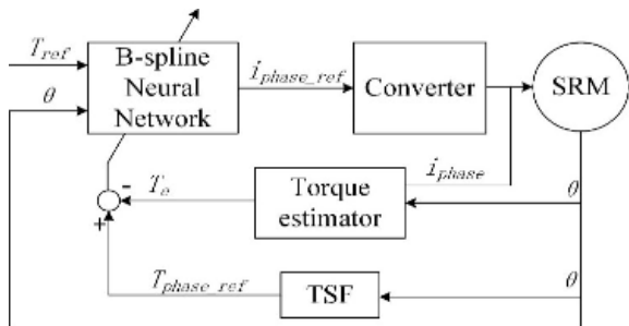
FIGURE 14. Diagram of B-spline neural network scheme [177].
