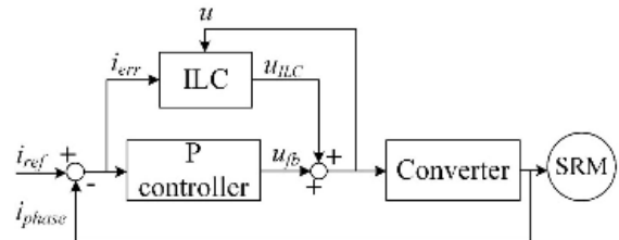
FIGURE 12. Block diagram for ILC-based current controller [173].
