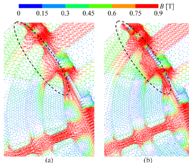
FIGURE 3. Flux density vectors of second-layer tapered flux barrier and common flux barrier in the worst conditions (1.5 times the maximum current, -40^{\circ}\text{C} ) [35]. (a) Common flux barrier. (b) Second layer tapered flux barrier.
