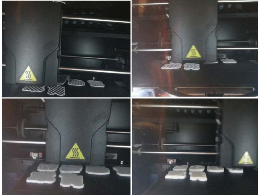
Figure 3. Laying down process of fused ABS polymer in typical FDM equipment.
