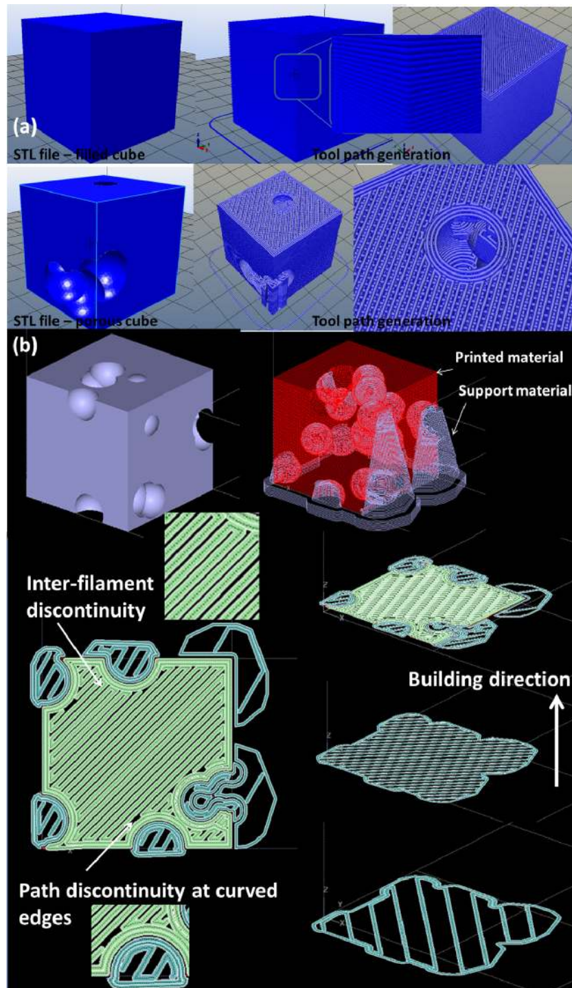
Figure 2. Typical examples of CAD objects transformed into collection of toolpaths using (a) Repetier and (b) CatalystEX software.
