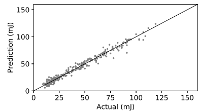
Figure 6. Energy predictor evaluation on Snapdragon 835 CPU.
