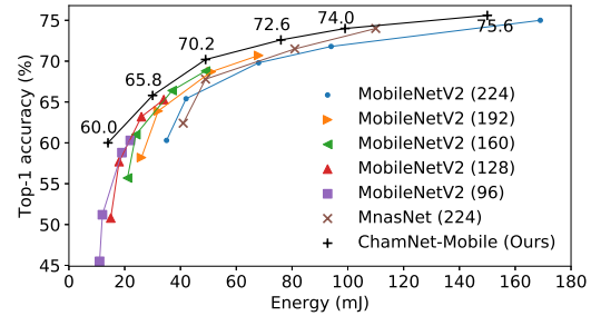
Figure 11. Energy-constrained ChamNet-Mobile on a Snapdragon 835 CPU.
