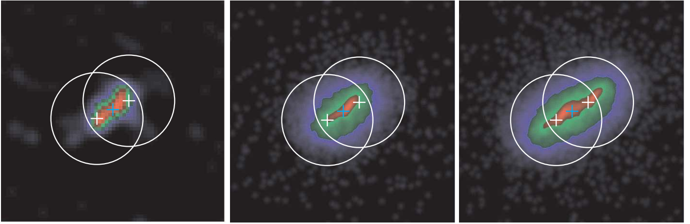
FIG. 3.—Large overlapping double X-ray sources detected by wavdetect (left), the PSF image at their median location (middle), and the combined image of two PSFs at each X-ray source position (right). The white crosses and circles mark the positions and sizes of the double sources. The cyan crosses indicate the median location of the double sources. Circle size corresponds to the source extraction region used in xapphot . The shape of the detected overlapping X-ray sources (left) are similar to the shape of the single PSF (middle), rather than double PSFs (right). We conclude that the overlapping X-ray sources are spurious doubles due to the elongated PSF shape and substructures in the PSF. The PSF images are generated by the ChaRT tool in the CIAO package and MARX package. The size of all images is \sim 30'' \times 30'' , and all images are aligned with the world coordinate system.
