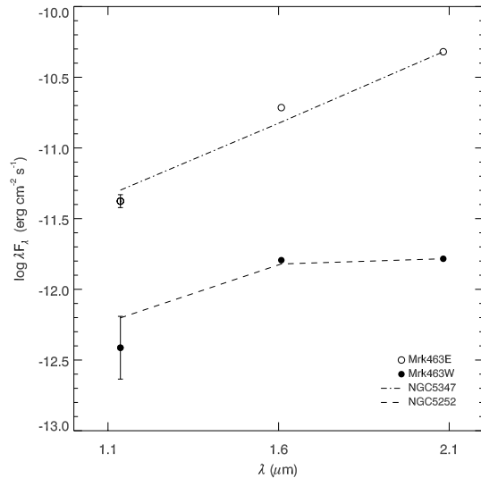
Figure 4. The HST NIR spectrum of the two nuclei in Mrk 463. In comparison, the HST NIR spectrum of type 2 Seyfert galaxies is plotted, renormalized at the 2.1- \mu\text{m} flux of the nuclei. See the text for details.
