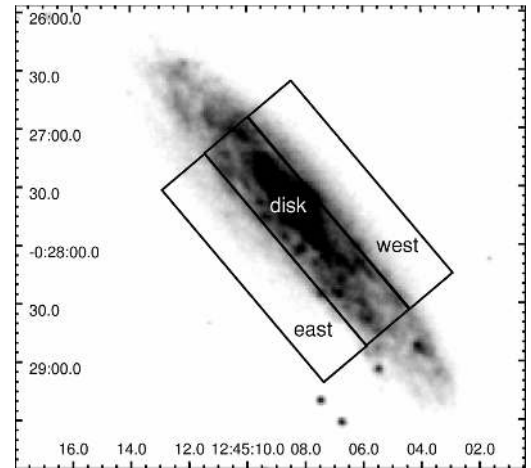
Fig. 5. The regions used for the spectral analysis of the disk of NGC 4666 on the DSS blue image.
