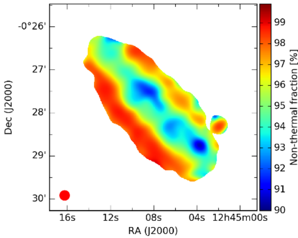
Fig. 18. NGC 4666 nonthermal fraction map at L-band. The beam of 13.3'' \times 13.3'' is shown in red (left bottom).
