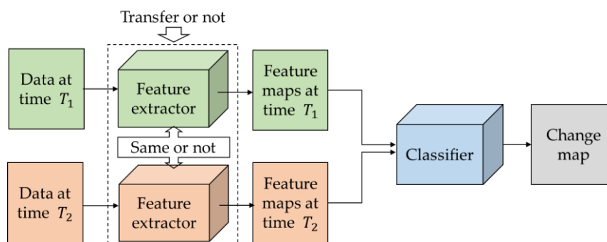
Figure 7. Schematic diagram of multi-model integrated structure of AI-based change detection.
