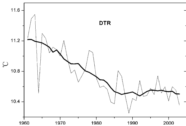
Fig. 6 Same as Fig. 4 but for DTR
