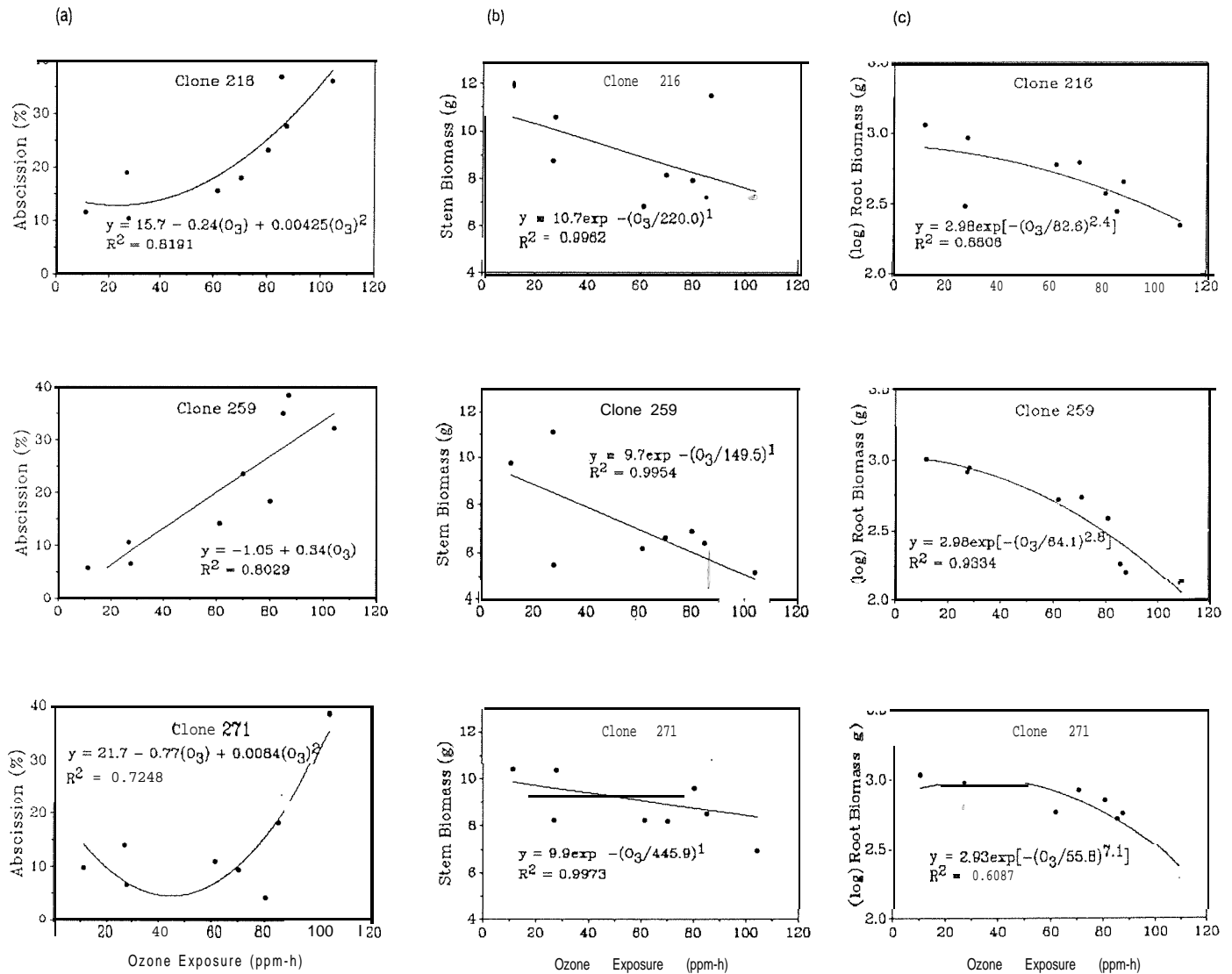
Fig. 2. Leaf abscission (a), stem biomass (b), and root biomass (c) responses to different total seasonal ozone exposures for three Populus tremuloides clones. Potted first-year plants were grown in open-top chambers and biomass was determined at the end of the 1991 growing season. The data points represent ozone exposures for individual chambers and are the mean of five plants per clone
