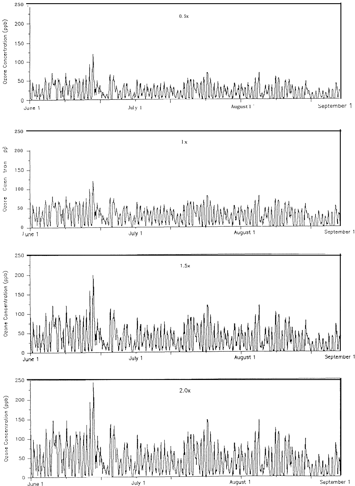
Fig. 1. Targeted ozone profiles for the month of June, July, and August. We used these as our targeted profiles in both 1990 and 1991. These profiles are based on modified ambient (1x) from southern Michigan. Sigmoidal weighting was used to develop the 0.5x, 1.5x, and 2x.
