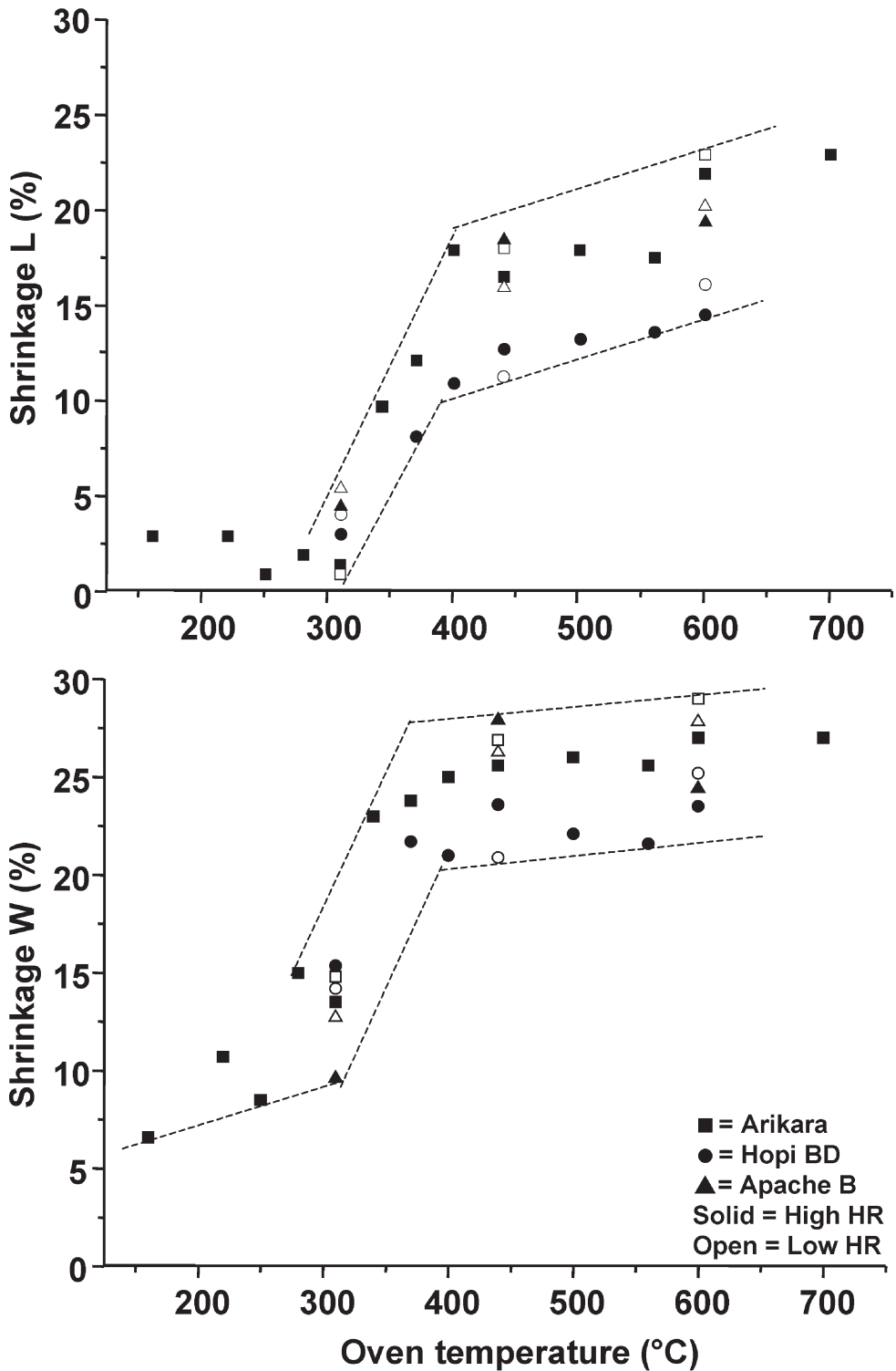
Fig. 5. Mean shrinkages of length (L) and width (W) of samples containing ten sunflower achenes of the indicated varieties as a function of the temperature in °C. Solid symbols carbonized at a high heating rate (HHR), open symbols at a low heating rate (LHR). Dashed lines indicate the upper and lower limits of the mean shrinkages.
