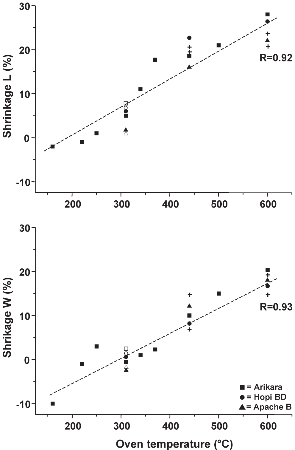
Fig. 7. Relationships between mean shrinkage of length (L) and width (W) of seeds of the three indicated varieties and the temperature in °C. The solid and open symbols represent high heating and low heating rates, respectively, and are carbonized after removal of the hull. Crosses (+) represent seeds carbonized in the hull at a low heating rate.
