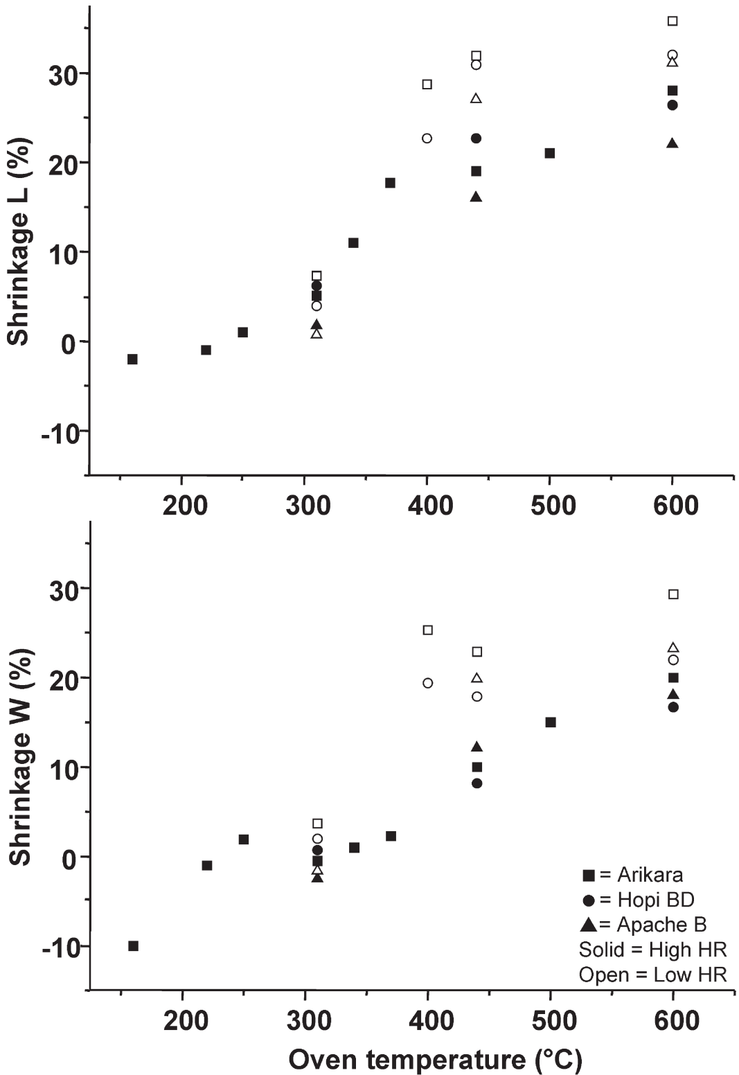
Fig. 4. Mean shrinkages of length (L) and width (W) of samples containing ten sunflower seeds of the indicated varieties as a function of the temperature in °C. Solid symbols carbonized at a high heating rate (HHR), open symbols at a low heating rate (LHR).
