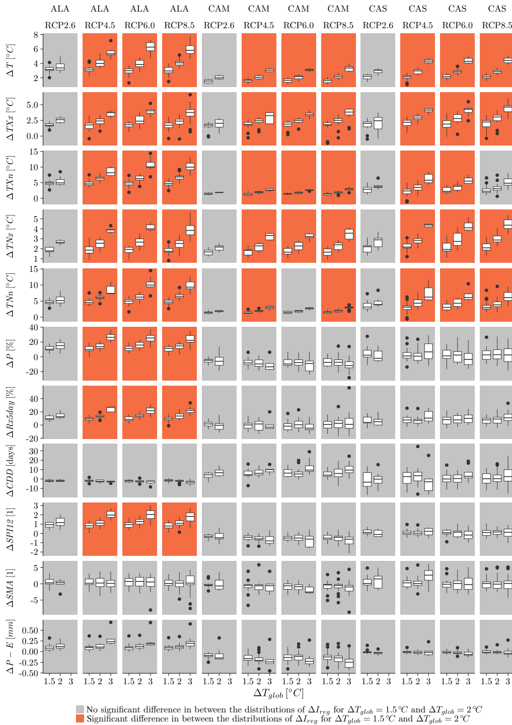
Figure A1. Response of indices \Delta T , \Delta T_{Xx} , \Delta T_{Xn} , \Delta T_{Nx} , \Delta T_{Nn} , \Delta P , \Delta R_{x5day} , \Delta CDD , \Delta SPI_{12} , \Delta SMA , and \Delta P - E to global mean temperature increases of 1.5, 2, and 3°C based on CMIP5 simulations of ensemble member r1i1p1 and averaged over the SREX regions ALA, CAM, and CAS. The upper and lower hinges of the box plots represent the first and third quartiles. The whiskers extend to the highest (lowest) value that is within 1.5 times the interquartile range of the upper (lower) hinge. The central line of each box plot indicates the median value. Values outside this range are displayed as dots. See Table 2 for a description of the indices.
