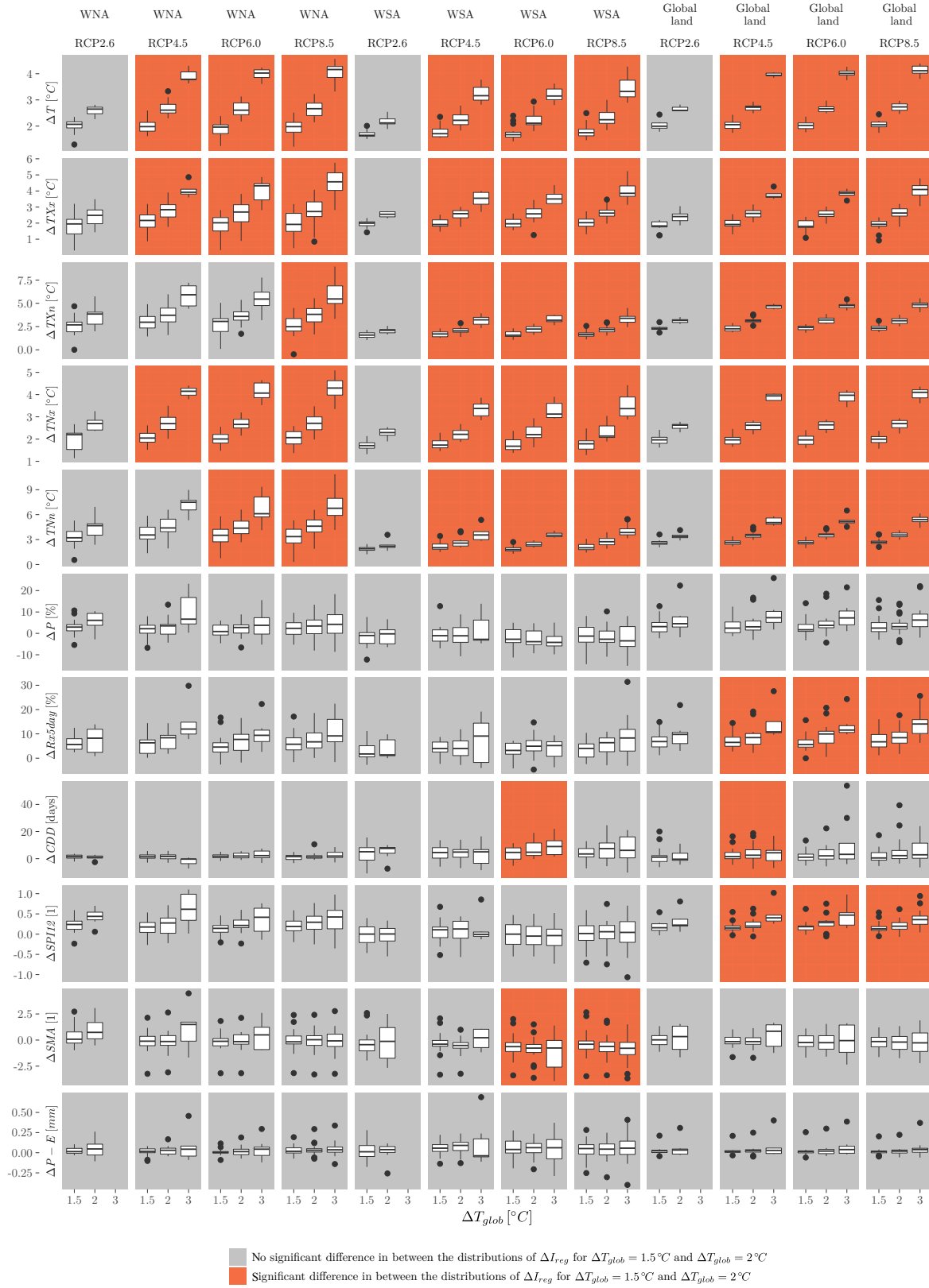
Figure A7. Like Fig. A1 but for SREX regions WNA and WSA, and for global land.
