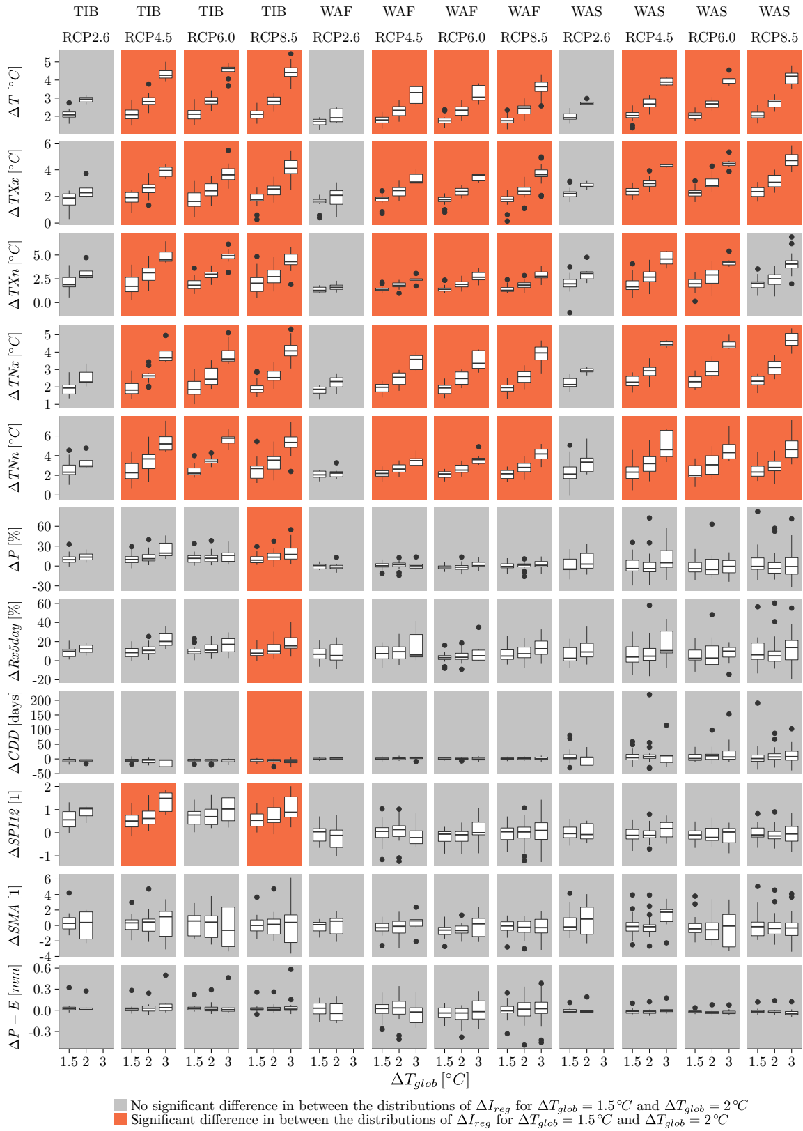
Figure A6. Like Fig. A1 but for SREX regions TIB, WAF, and WAS.
