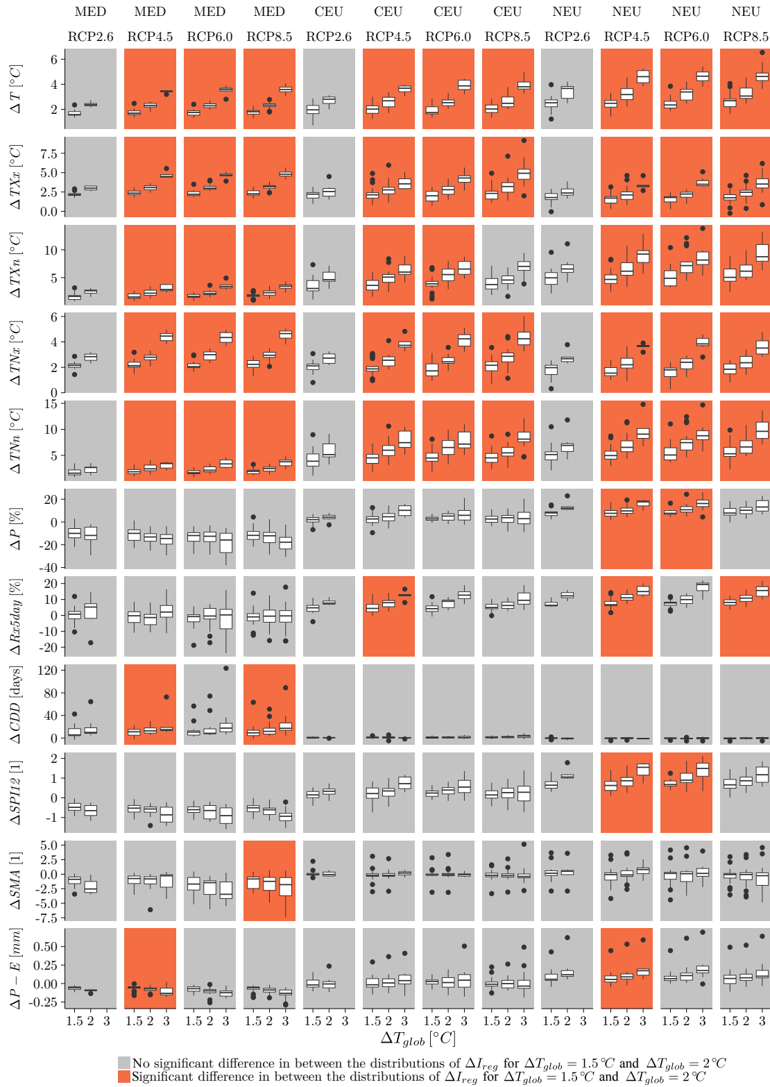
Figure 5. Response of indices \Delta T , \Delta T_{Xx} , \Delta T_{Xn} , \Delta T_{Nx} , \Delta T_{Nn} , \Delta P , \Delta Rx5day , \Delta CDD , \Delta SPI12 , \Delta SMA , and \Delta P - E to a global mean temperature increase of 1.5, 2, and 3°C based on CMIP5 simulations of ensemble member r1i1p1 and averaged over the European SREX regions MED, CEU, and NEU. The upper and lower hinges of the box plots represent the first and third quartiles. The whiskers extend to the highest (lowest) value that is within 1.5 times the interquartile range of the upper (lower) hinge. The central line of each box plot indicates the median value. Values outside this range are displayed as dots.
