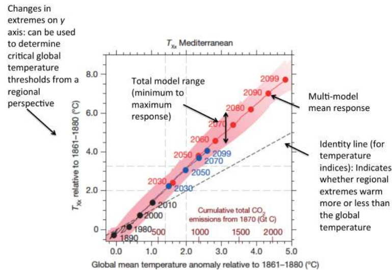
Figure 1. Example of a plot displaying the functional relationship of a regional climate index (annual maximum of daily maximum temperature, T_{Xx} ) on global mean temperature following the S16 approach, including explanatory annotations (adapted from S16).
