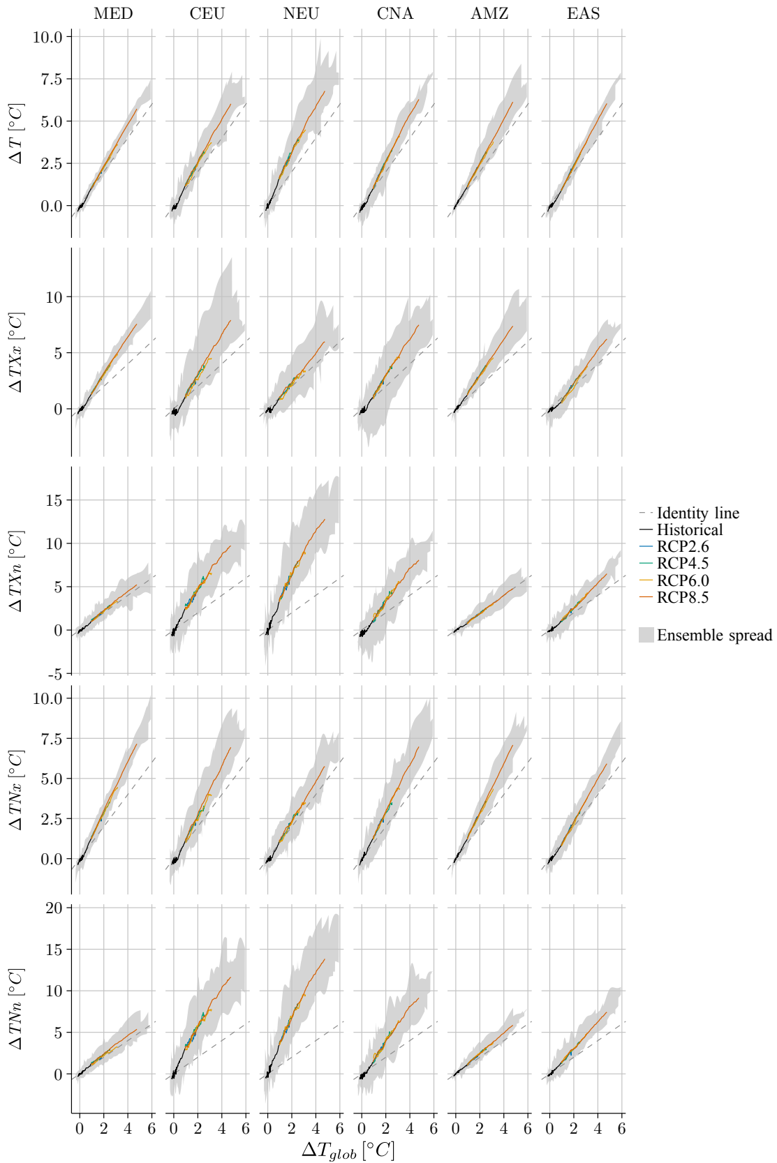
Figure 3. Functional relationships with global mean temperature for the indices \Delta T , \Delta T_{Xx} , \Delta T_{Xn} , \Delta T_{Nx} , and \Delta T_{Nn} , based on CMIP5 simulations of ensemble member r1i1p1 and averaged over the SREX regions MED, CEU, NEU, CNA, AMZ, and EAS. See Table 2 for a description of the indices.
