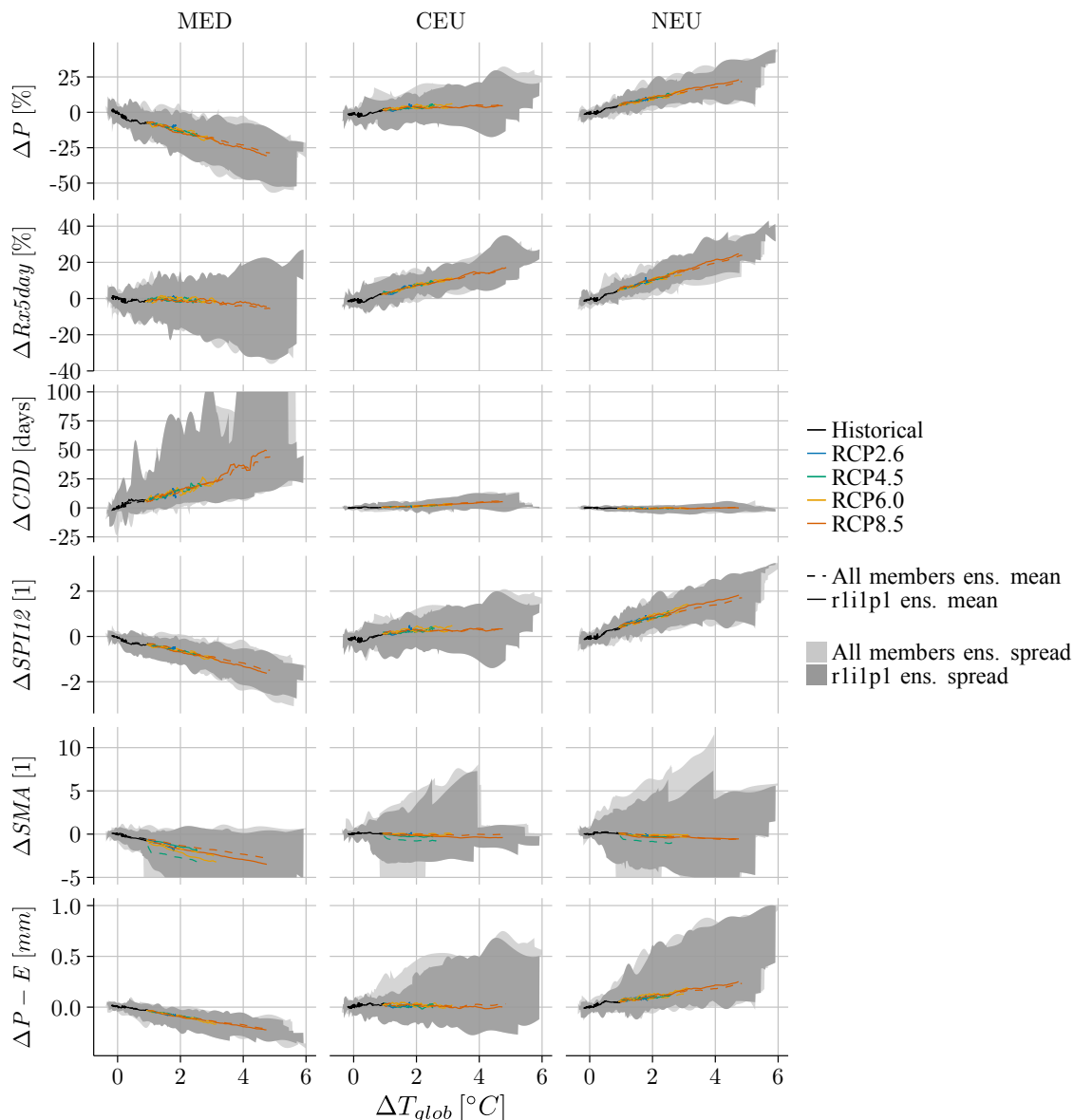
Figure 8. Functional relationships with global mean temperature for the indices \Delta P , \Delta R_{rx5day} , \Delta CDD , \Delta SPI_{12} , \Delta SMA , and \Delta P - E , averaged over the SREX regions MED, CEU, and NEU. Indices based on all CMIP5 ensemble members available per model (solid lines, dark shading) are compared with indices based on ensemble member r1i1p1 of each model (dashed lines, light shading). Values for \Delta CDD > 100 days and \Delta SMA < -5 were cut off for readability.
