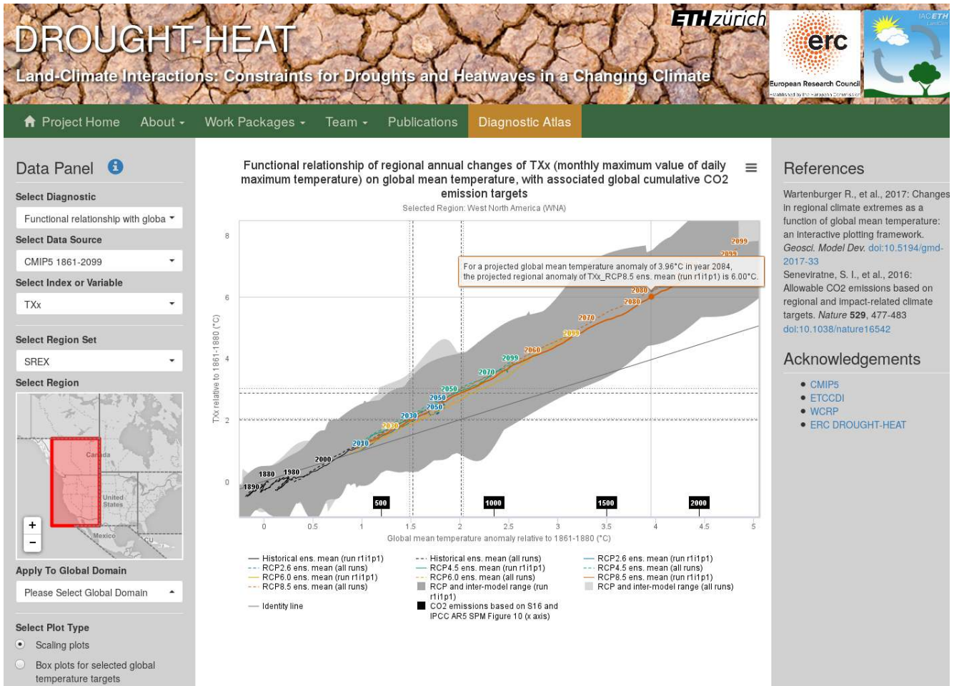
Figure 2. Screenshot of the DROUGHT-HEAT Regional Climate Atlas. For demonstration, this screenshot displays the functional relationship of \Delta T_{Xx} on \Delta T_{\text{glob}} based on model simulations from 1861 to 2099 for the SREX region west North America (WNA).
