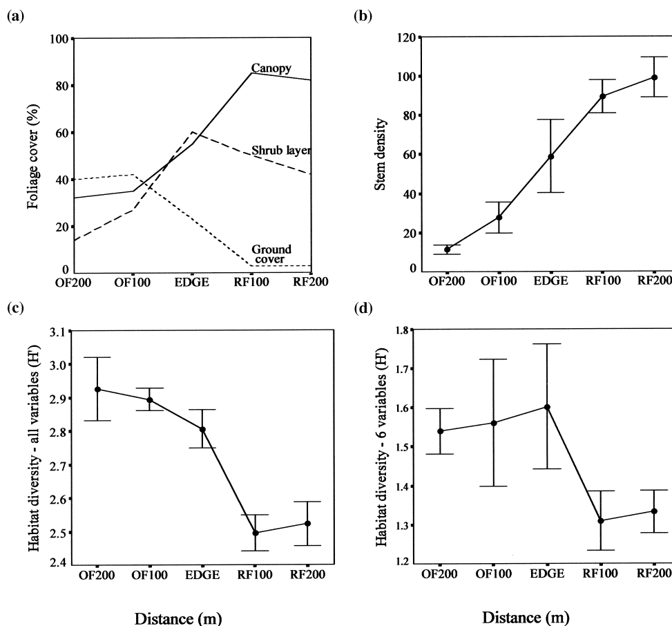
Figure 1. Changes in the vegetation structure across the rain forest ecotone at Paluma sites 1 and 2 (Error bars are 95% confidence intervals): (a) trends in foliage density of the canopy (>5 m), shrub layer (1–5 m) and ground cover (<1 m); (b) stem density measured by the number of trees (>3 m high) per 100 m 2 ; (c) Shannon index H' based on all habitat variables; (d) Shannon index H' based on six structural attributes of vegetation. Position on the ecotonal gradient is indicated by: OF200 – open forest grids 200 m from the rain forest edge; OF100 – open forest grids 100 m from the rain forest edge; EDGE – grids on the rain forest/wet sclerophyll forest boundary; RF100 – grids 100 m into the rain forest; RF200 – grids 200 m into the rainforest.
