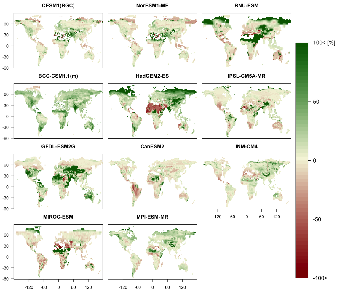
Fig. 3. Relative change in soil carbon density (%) over the 21st century for all models (difference in 10-year means divided by modern soil carbon density; 2090–2099 minus 1997–2006 divided by 1997–2006).
