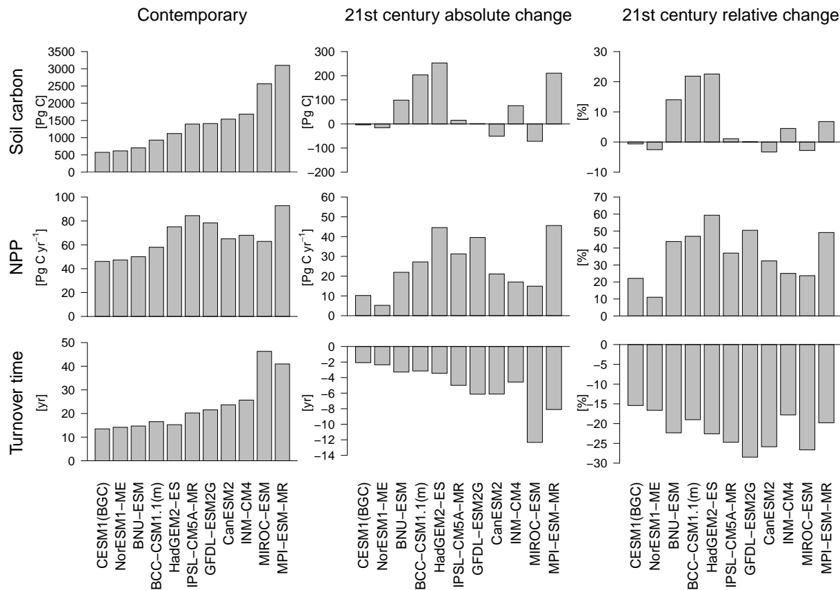
Fig. 1. Contemporary values, absolute changes, and relative changes of soil carbon, net primary production (NPP), and turnover times for CMIP5 Earth system models. Contemporary values of soil carbon, NPP, and turnover times are reported for the 1997–2006 mean using model output from the historical experiment. Changes for the 21st century were estimated from the difference between 2090–2099 and 1997–2006 mean model estimates from the RCP 8.5 experiment. Turnover times were calculated from global soil carbon stocks divided by global heterotrophic respiration.
