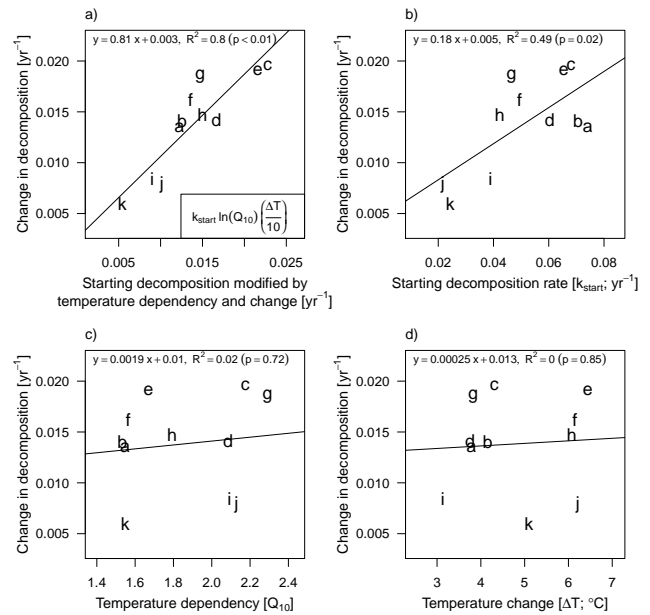
Fig. 7. Change in decomposition rate between 1997–2006 and 2009–2009 global means due to variation in (a) starting decomposition rate, Q_{10} , and soil temperature change from Eq. (7), k_{\text{start}} \ln(Q_{10}) \left(\frac{\Delta T}{10}\right) , (b) starting decomposition rate, k_{\text{start}} , (c) temperature dependency, Q_{10} , and (d) change in soil temperature, \Delta T . The models are represented as follows; a: CESM1(BGC), b: NorESM1-ME, c: BNU-ESM, d: BCC-CSM1.1(m), e: HadGEM2-ES, f: IPSL-CM5A-MR, g: GFDL-ESM2G, h: CanESM2, i: INM-CM4, j: MIROC-ESM, and k: MPI-ESM-MR.
