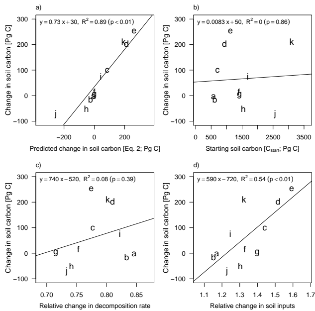
Fig. 6. Change in global soil organic carbon between 1997–2006 and 2090–2099 global means as a function of (a) Eq. (2), the relative change in input and decomposition rate times the initial soil carbon stock, \left(\frac{1 + \frac{\Delta I}{I_{\text{start}}}}{1 + \frac{\Delta k}{k_{\text{start}}}} - 1\right) \times C_{\text{start}} , (b) starting soil carbon stock, C_{\text{start}} , (c) the inverse of the relative change in decomposition rate ( k ), \frac{1}{1 + \frac{\Delta k}{k_{\text{start}}}} , and (d) relative change in soil inputs ( I ), 1 + \frac{\Delta I}{I_{\text{start}}} . The models are represented as follows; a: CESM1(BGC), b: NorESM1-ME, c: BNU-ESM, d: BCC-CSM1.1(m), e: HadGEM2-ES, f: IPSL-CM5A-MR, g: GFDL-ESM2G, h: CanESM2, i: INM-CM4, j: MIROC-ESM, and k: MPI-ESM-MR.
