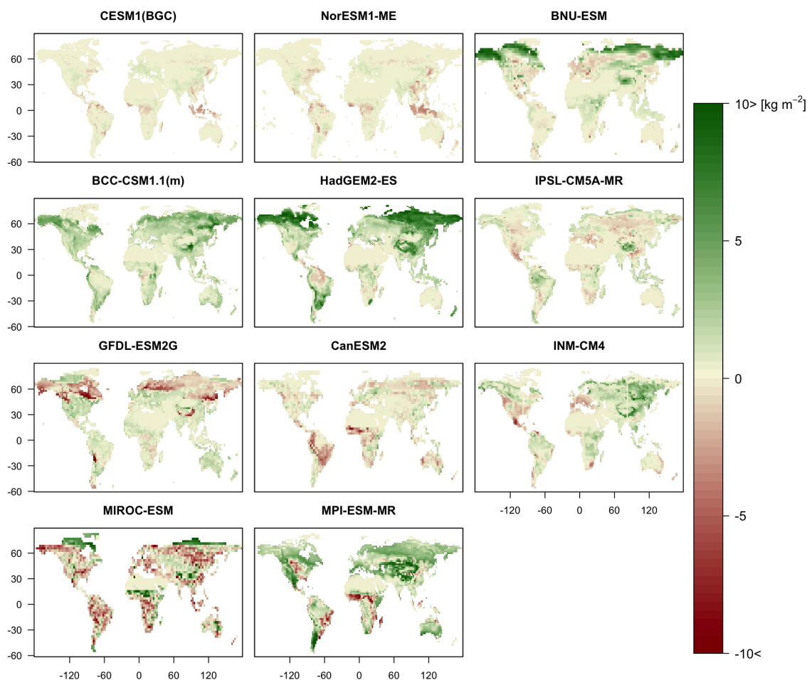
Fig. 2. Absolute change in soil carbon density ( \text{kg m}^{-2} ) over the 21st century for all models (difference in 10-year means; 2090–2099 minus 1997–2006).
