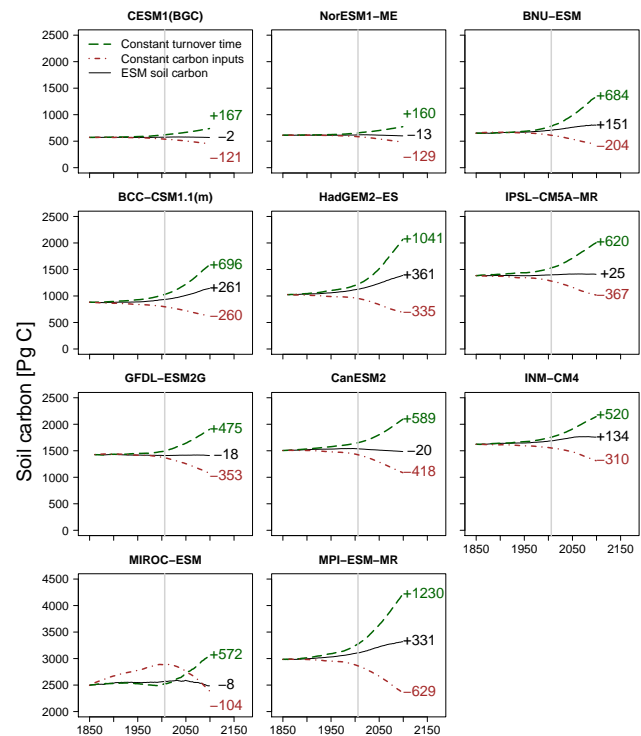
Fig. 5. Soil carbon over time (historical and RCP 8.5) under the “constant turnover time” and “constant carbon inputs” scenarios. The black solid line is the ESM-simulated global soil carbon stock with the net change from 1850 indicated in black text. The green dashed line is the soil carbon stock that would be predicted if turnover time were held constant at the 1850 value and soil inputs were allowed to evolve as predicted by the ESM, with the net change indicated in green text. The red dotted line is the soil carbon stock that would be predicted if carbon inputs were held constant at 1850 levels and the turnover time were allowed to evolve as predicted by the ESM, with the net change in red text. The vertical grey line at 2006 indicates where the historical experiment ends and the RCP 8.5 experiment begins.
