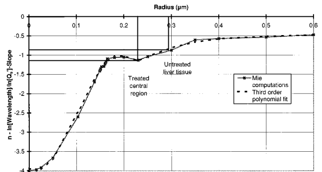
Fig. 8. Deduced slope coefficients from the Q_s' spectra calculated on the Mie theory, as shown in Fig. 7, corresponding to the wavelength exponent n versus the particle radius. A mathematical fit was deduced, composed of two polynomials of the third order, and is represented by the dashed curve. The slight hump in the range r = 0.15\text{--}0.20 \mu\text{m} can be explained by an overestimation of the wavelength exponent, as the linear regression fit is not optimal for these intermediate-sized particles, as shown in Fig. 7.
