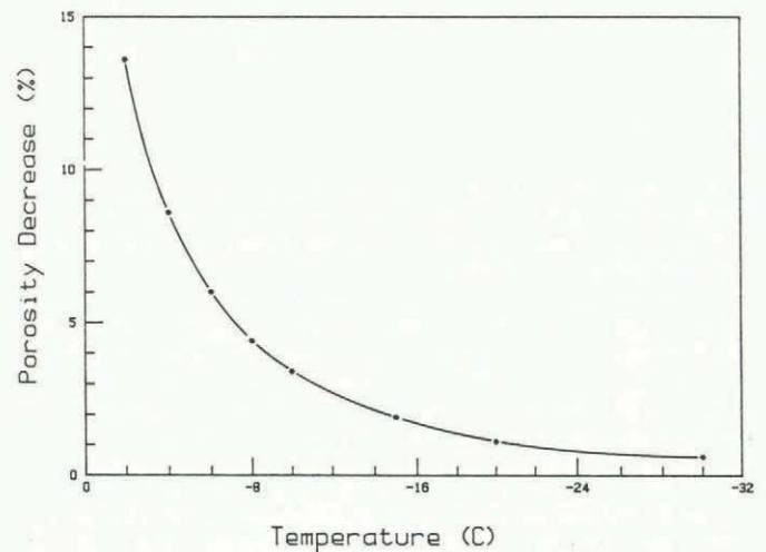
Fig. 2. Porosity decrease of ice samples cycled from different in-situ temperatures to -54^{\circ}\text{C} and then returned to the initial in-situ temperature.
