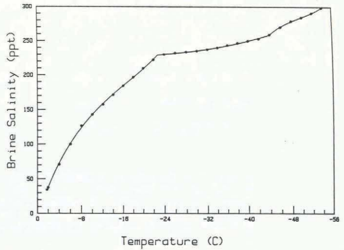
Fig. 1. Brine salinity versus ice temperature. The line represents least-squares curve fits through the data.
