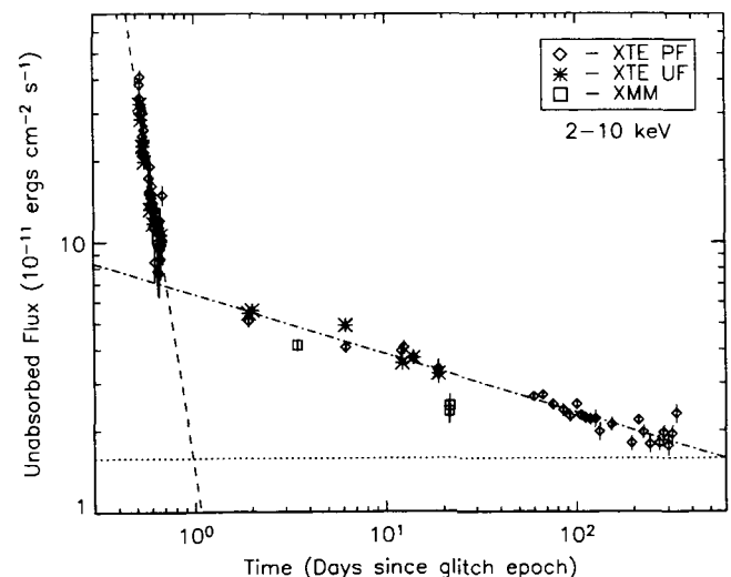
Fig. 13.—Time evolution of the unabsorbed flux from 1E 2259+586 following the 2002 June outburst. The glitch epoch (Table 4) is used as the reference time for this plot. Diamonds denote inferred unabsorbed flux values calculated from RXTE PCA pulsed-flux measurements. Asterisks and squares mark independent phase-averaged unabsorbed flux values from RXTE and XMM-Newton , respectively. The dotted line denotes the flux level measured using XMM-Newton 1 week prior to the glitch. The dashed line is a power-law fit to the PCA flux measurements during the observations containing the burst activity (<1 day). The dot-dashed line marks the power-law fit to all data more than 1 day following the glitch. See text for further details.
