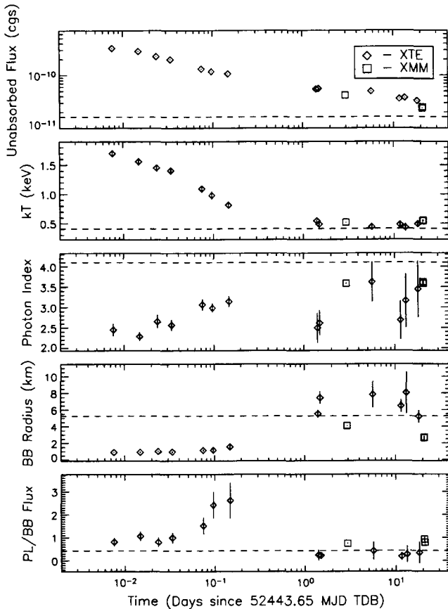
Fig. 12.—Spectral evolution of 1E 2259+586 through and following the outburst of 2002. Top to bottom : Unabsorbed flux (2–10 keV), the blackbody temperature ( kT ), the photon index, the blackbody radius, and the ratio of power-law (2–10 keV) to bolometric blackbody flux. A distance of 3 kpc was assumed (Kothes, Uyaniker, & Aylin 2002) to compute the blackbody radius. Horizontal dashed lines denote the values of each parameter during the XMM-Newton observation 1 week prior to the outburst.
