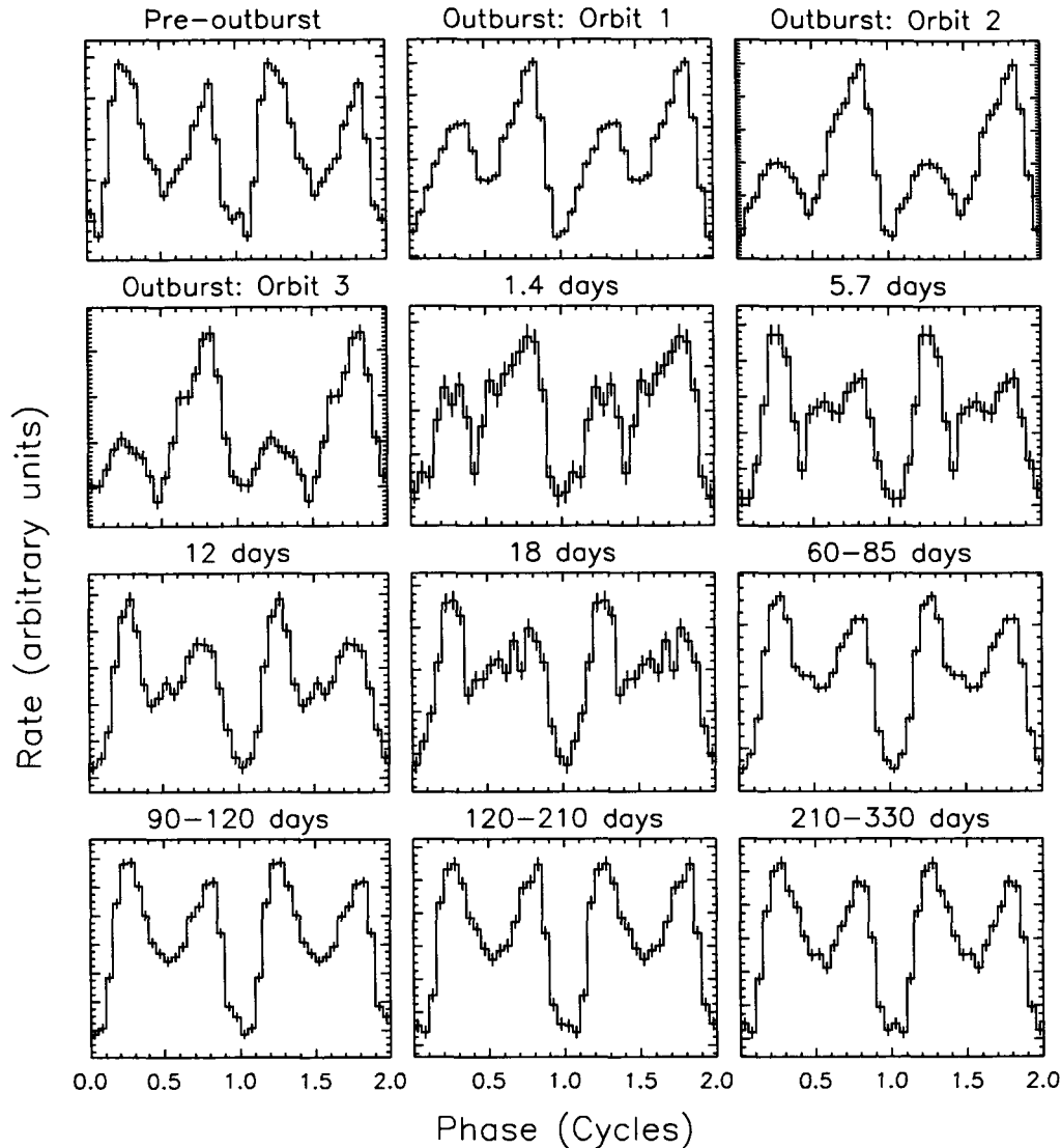
FIG. 10.—Time evolution of the 2–10 keV pulse profile of 1E 2259+586 through the outburst of 2002. Profiles have arbitrary flux units, and two pulse cycles are shown for clarity. Time increases from left to right and top to bottom.
