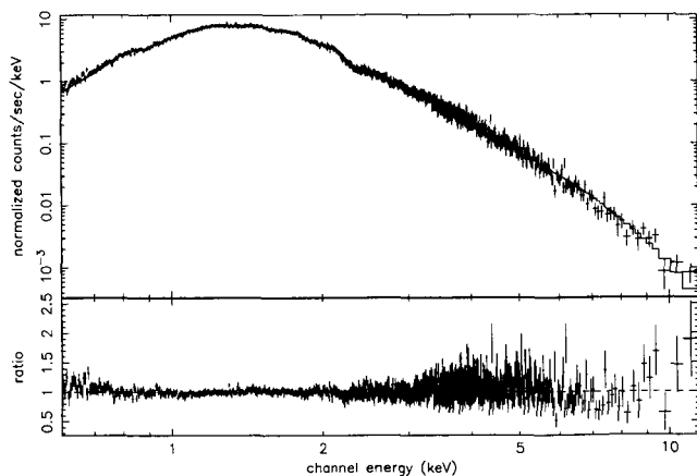
FIG. 2.—Phase-averaged X-ray spectrum of 1E 2259+586 as observed with the XMM-Newton pn camera during the observation 1 week prior to the 2002 June outburst (Obs2). Bottom , Ratio of the data to the best-fit model (see Table 3) folded through the instrumental response.
