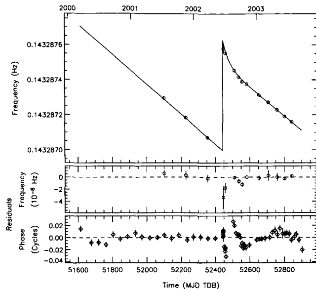
FIG. 6.— Top : Frequency evolution of 1E 2259+586 around the time of the outburst for a simple exponential recovery model. See text for details. The line represents the best-fit model. The circles denote frequency measurements for independent subsets of data. Middle : Frequency residuals of the independent frequency points minus the model. Bottom : Phase residuals with respect to the best-fit model. Clearly, there is a systematic trend in the postglitch residuals reflecting the inadequacy of this model.
