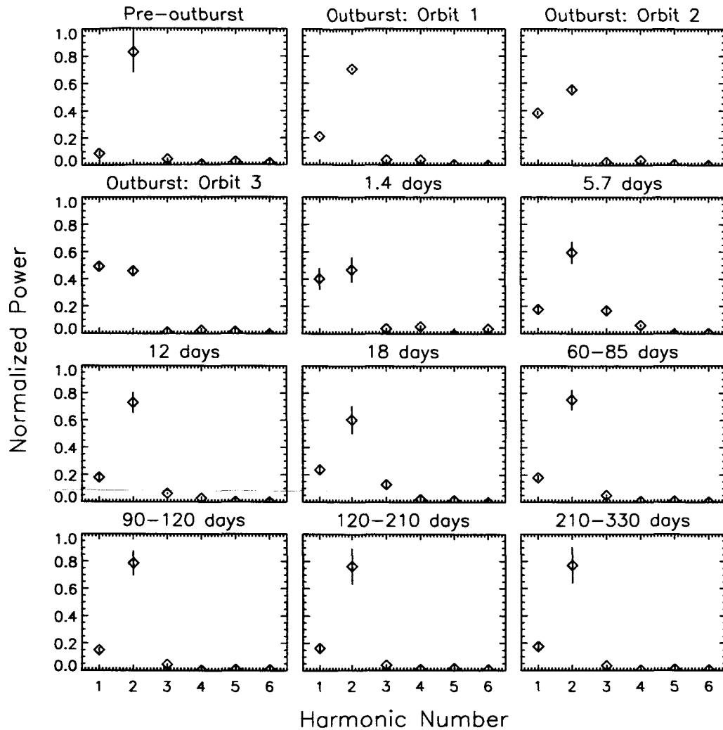
FIG. 11.—Time evolution of the Fourier power harmonic distribution of the 2–10 keV pulse profile of 1E 2259+586 through the outburst of 2002. Power levels have been normalized to the total power of the first seven harmonics. Time increases from left to right and top to bottom.
