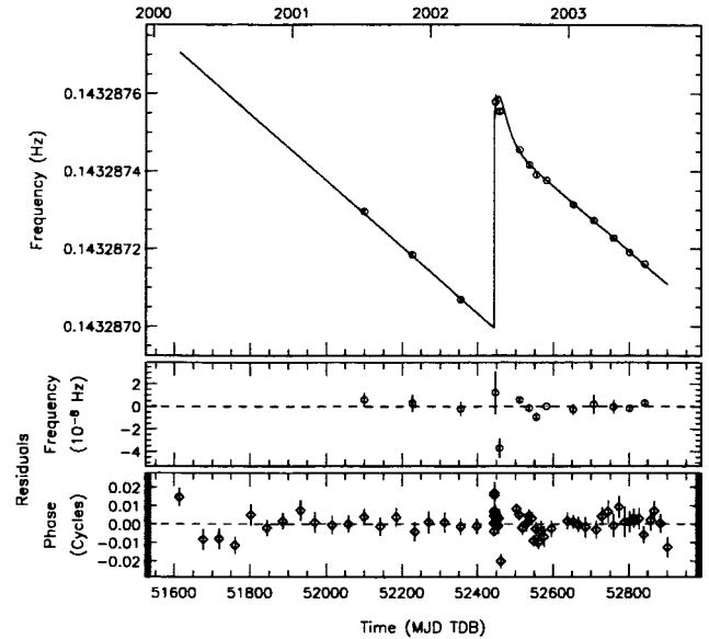
FIG. 7.— Top : Frequency evolution of 1E 2259+586 around the time of the outburst for a model including an exponential rise and fall in frequency postglitch. See text for details. The line represents the best-fit model (see Table 4 for model parameters). The circles denote frequency measurements for independent subsets of data. The effect of the glitch is obvious, as is the partial recovery. Middle : Frequency residuals of the independent frequency points minus the model. Bottom : Phase residuals with respect to the best-fit model. Closer inspection of the residual cluster just following the outburst epoch reveals a low-amplitude systematic trend. This is discussed further in the text.
