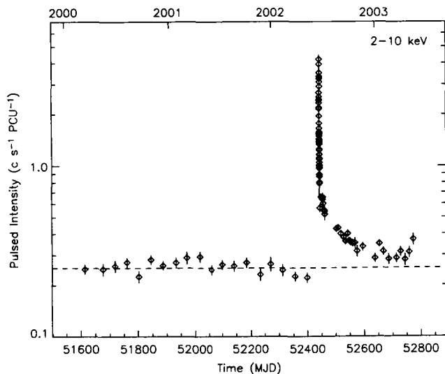
FIG. 8.—Pulsed-flux history of 1E 2259+586 (2–10 keV) from 2000 March through 2003 June as measured using the RXTE PCA. The sharp rise in the pulsed intensity coincides with the burst activity.
