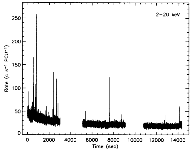
FIG. 5.— RXTE PCA light curve of 1E 2259+586 recorded on 2002 June 18. The light curve displays counts within 2–20 keV at 1 s time resolution.
