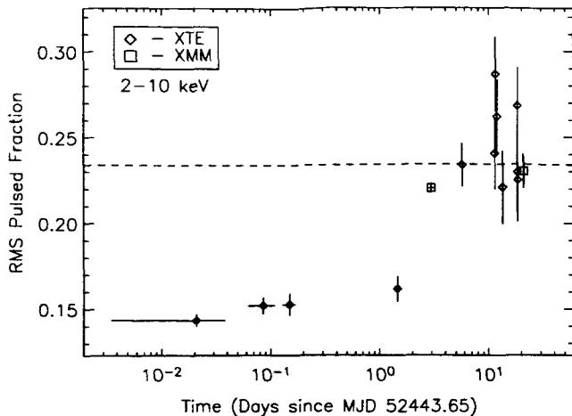
Fig. 9.—Time evolution of the 2–10 keV pulsed fraction of 1E 2259+586 through the outburst of 2002 showing measurements made with the RXTE PCA (diamonds) and XMM-Newton measurements (squares; Table 2). The horizontal dashed line marks the pulsed fraction from the XMM-Newton observation 1 week prior to the outburst (Obs2).
