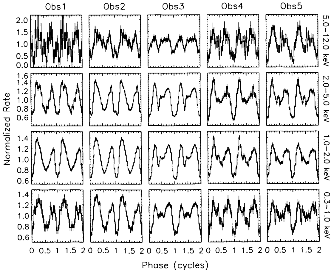
FIG. 1.—Folded-pulse profile of 1E 2259+586 as observed with the XMM-Newton pn camera as a function of energy for the all five observations. Time increases from left to right. The burst activity is recorded between Obs2 and Obs3. See Table 1 for exact times of observations.
