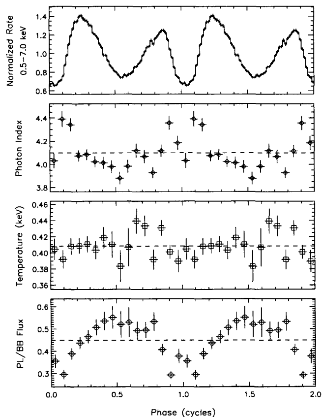
FIG. 3.—Phase-resolved X-ray spectrum of 1E 2259+586 as observed with the XMM-Newton pn camera 7 days prior to the observed burst activity (Obs2). Top to bottom : Folded pulse profile over the energy range 0.5–7.0 keV, the photon index, the blackbody temperature ( kT ), and the ratio of power-law to blackbody flux. The horizontal dashed lines in the bottom three panels denote the average value for each spectral parameter. For the ratio of power-law to blackbody flux, the power-law flux was summed over the energy range 2–10 keV, and the blackbody was summed over all photon energies, each corrected for the interstellar absorption (see text for value).
