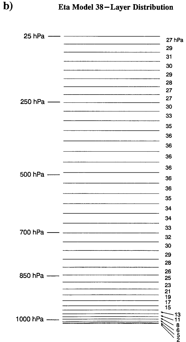
FIG. 1. (b) The distribution of the 38 layers in the 48-km eta model. The pressures on the left side indicate the layers' positions with respect to the standard atmosphere, while the numbers on the right give an approximate pressure depth of each layer in hectopascals.
