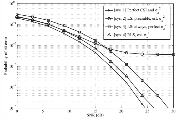
Fig. 5. Probability of bit error for SC-FDE systems employing various channel estimation/tracking techniques in a channel with a normalized Doppler spread of f_n = 1.5 \times 10^{-6} .
