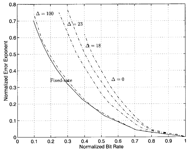
Fig. 6. Error exponent of variable input scheme at various feedback delays \Delta (in number of symbols).
