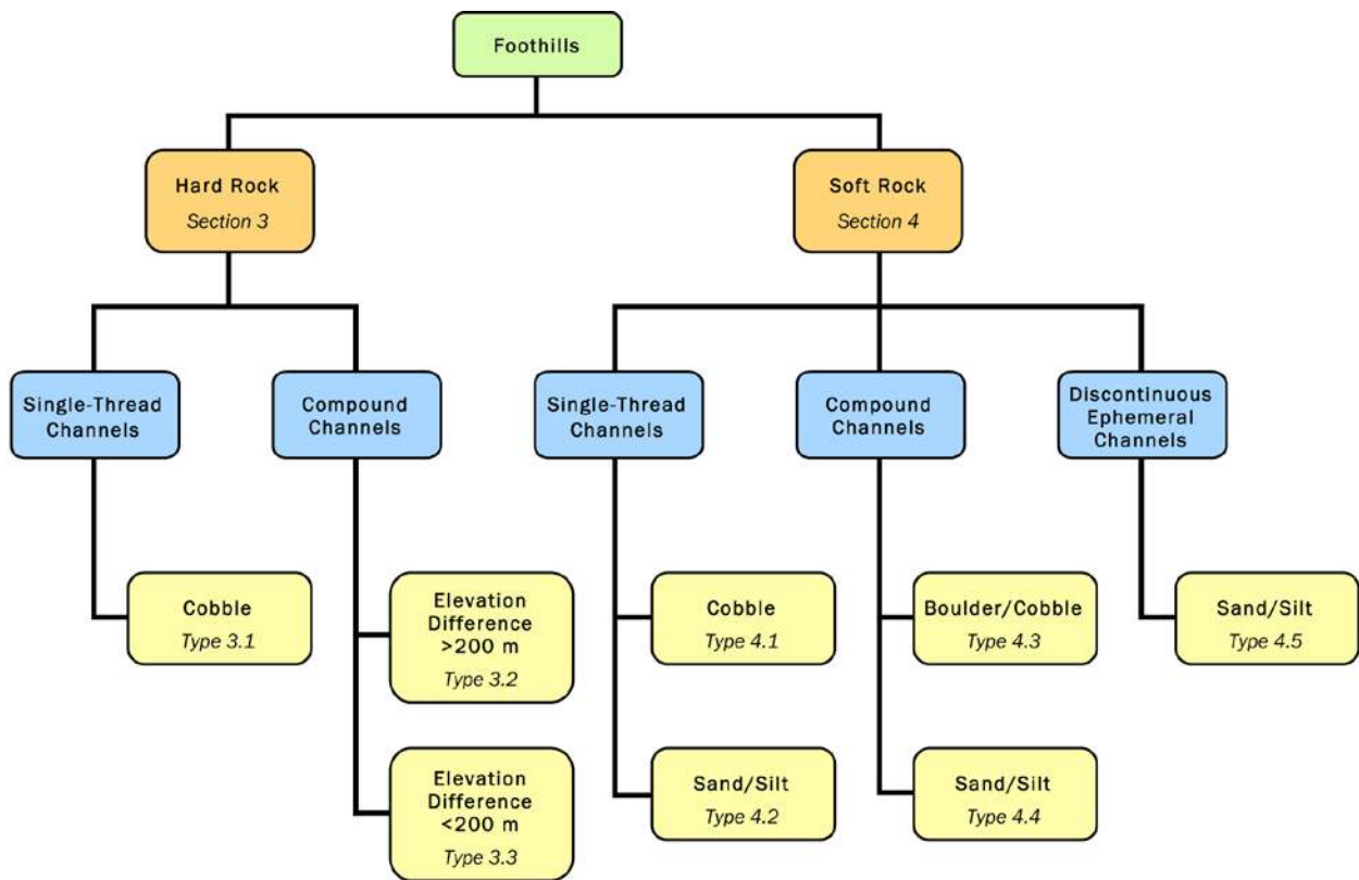
Figure 23. Classification of foothill channels in the Arid West region. In the following descriptions, headings for the orange boxes are bold, blue boxes bold italics, and yellow boxes italics.
