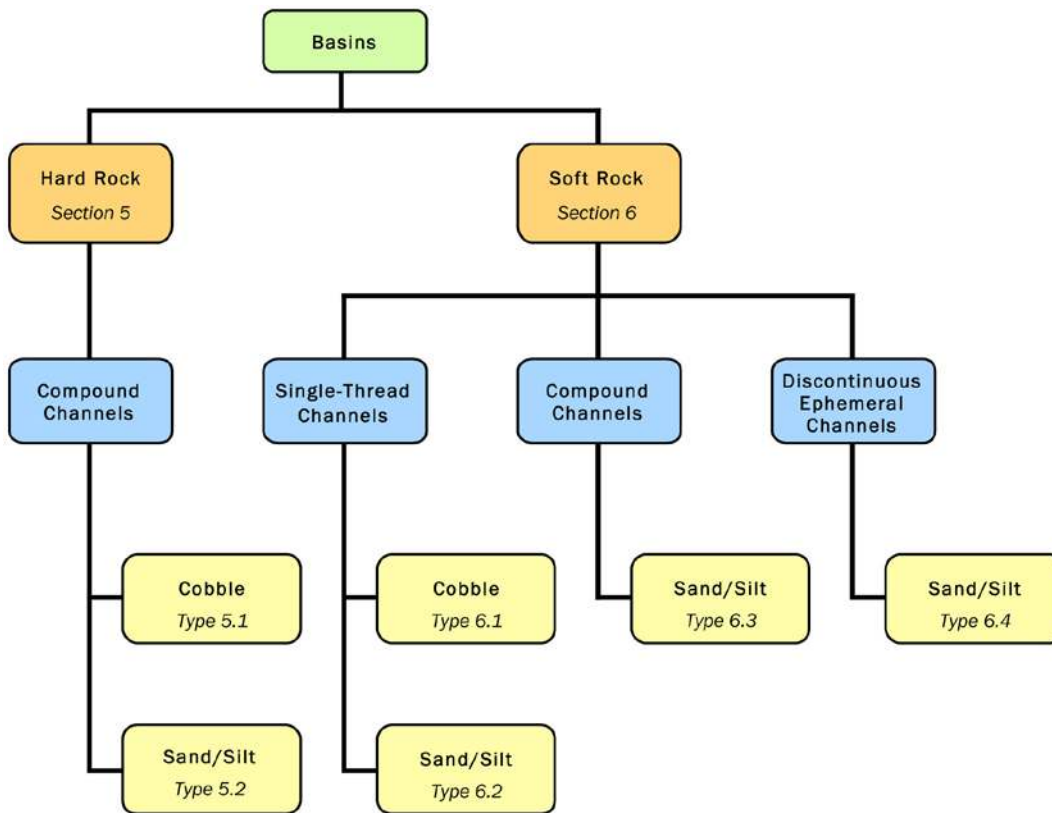
Figure 43. Classification of basin channels in the Arid West region. In the following descriptions, headings for the orange boxes are bold, blue boxes bold italics, and yellow boxes italics.
