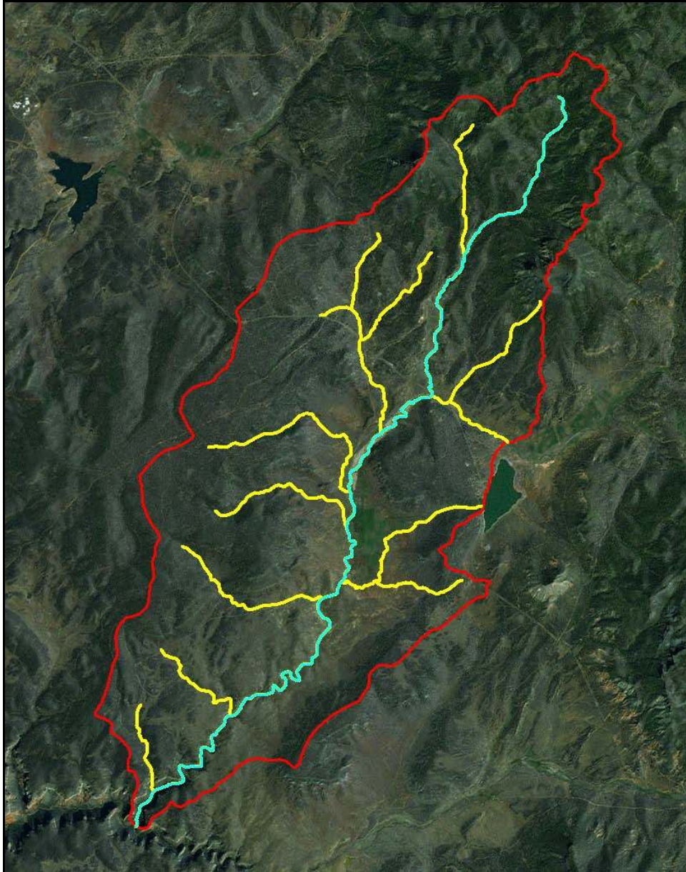
Figure 5. National Hydrography Dataset for Chinle Creek, AZ (red: boundary of watershed; yellow: stream channel data; blue: principal flow path).
