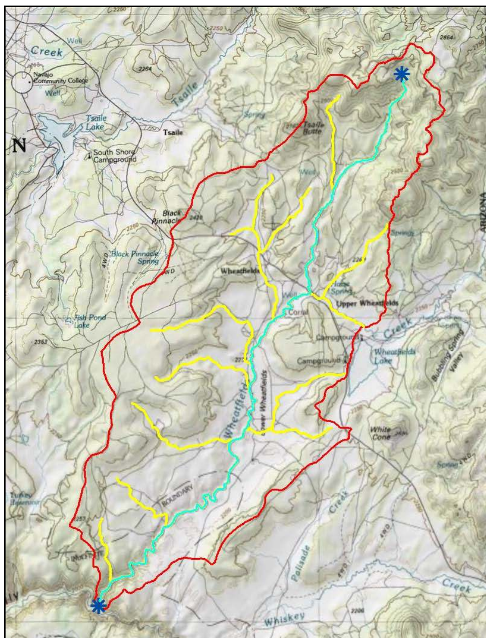
Figure 6. Example of elevation difference determined from the principal flow path at Chinle Creek, AZ (red: boundary of watershed; yellow: stream channel data; blue: principal flow path; blue stars: highest and lowest points of the principal flow path).
