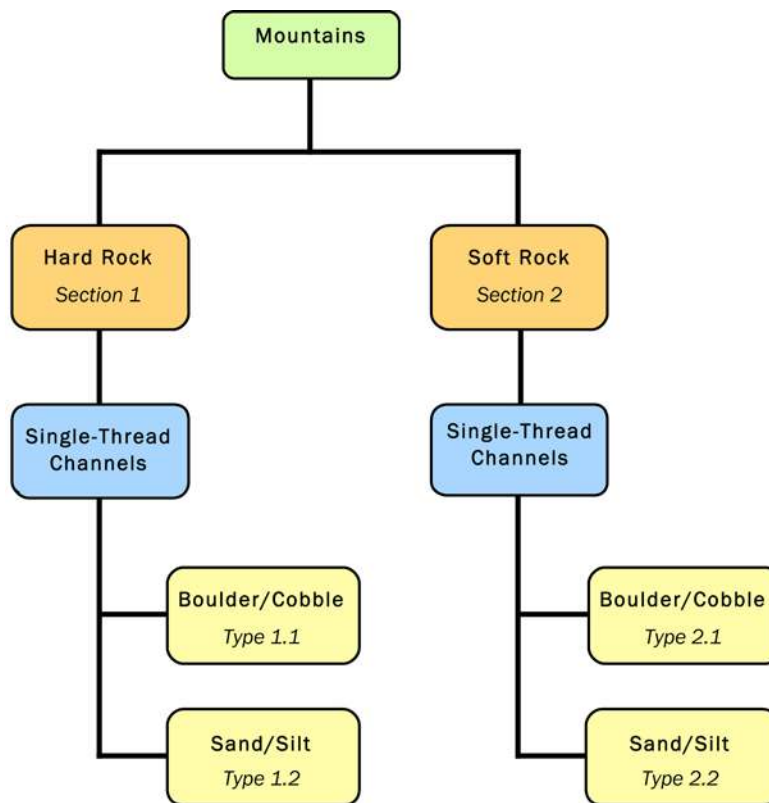
Figure 10. Classification of mountain channels in the Arid West region. In the following descriptions, headings for the orange boxes are bold, blue boxes bold italics, and yellow boxes italics.
