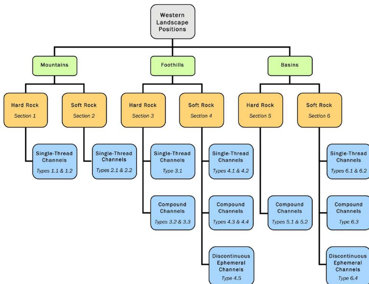
Figure 9. Channel classification for the Arid West region in support of OHW delineations (green: landscape position; orange: geology; blue: channel morphology).
